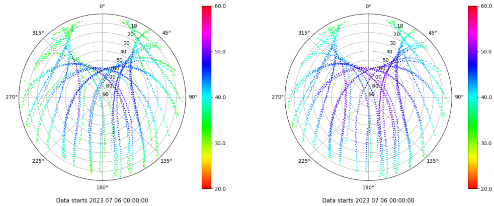
Skyplot for station ZARA. Signal to Noise S1C Data file ZARA00ESP_R_2023187.xtr Skyplot for station ZARA. Signal to Noise S2C Data file ZARA00ESP_R_2023187.xtr
