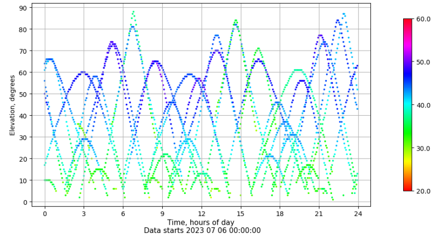
Time-elevation plot for station ZARA. Signal to Noise S1C Data file ZARA00ESP_R_2023187.xtr
