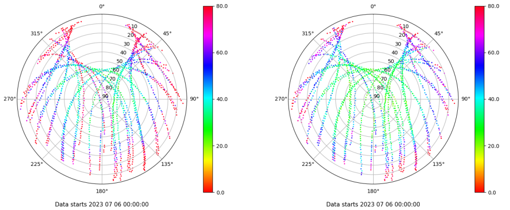
Skyplot for station ZARA. Parameter M1C Data file ZARA00ESP_R_2023187.xtr Skyplot for station ZARA. Parameter M2C Data file ZARA00ESP_R_2023187.xtr
