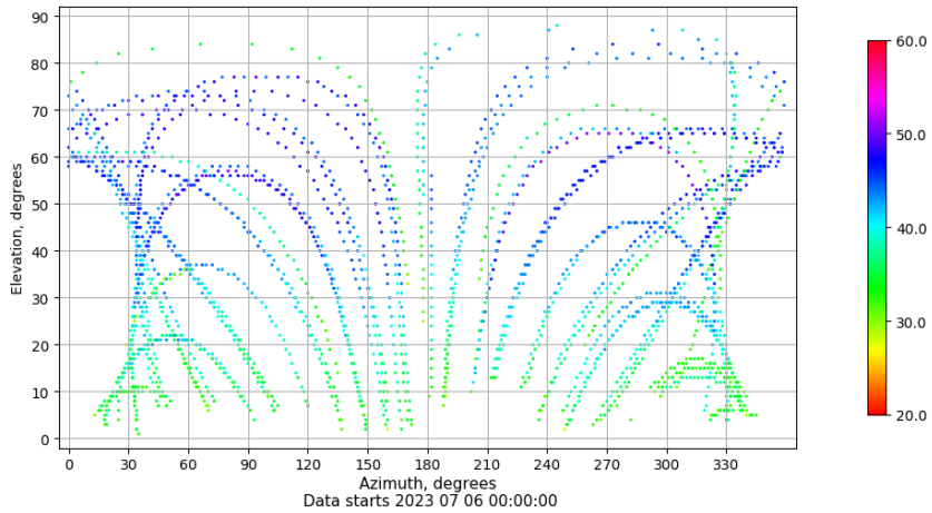
Azimuth-elevation plot for station ZARA. Signal to Noise S1C Data file ZARA00ESP_R_2023187.xtr
