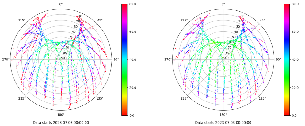
Skyplot for station ZARA. Parameter M1C Data file ZARA00ESP_R_2023184.xtr Skyplot for station ZARA. Parameter M2C Data file ZARA00ESP_R_2023184.xtr
