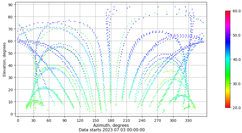
Azimuth-elevation plot for station ZARA. Signal to Noise S1C Data file ZARA00ESP_R_2023184.xtr
