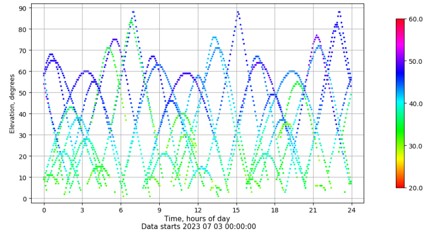
Time-elevation plot for station ZARA. Signal to Noise S1C Data file ZARA00ESP_R_2023184.xtr
