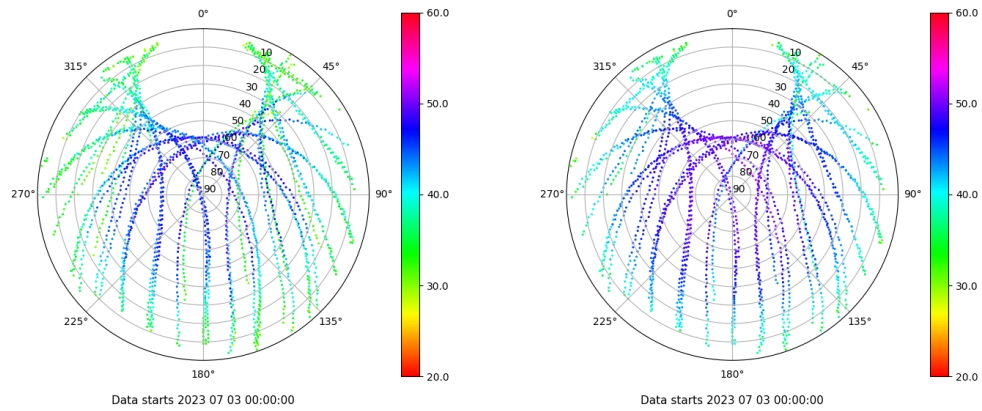
Skyplot for station ZARA. Signal to Noise S1C Data file ZARA00ESP_R_2023184.xtr Skyplot for station ZARA. Signal to Noise S2C Data file ZARA00ESP_R_2023184.xtr
