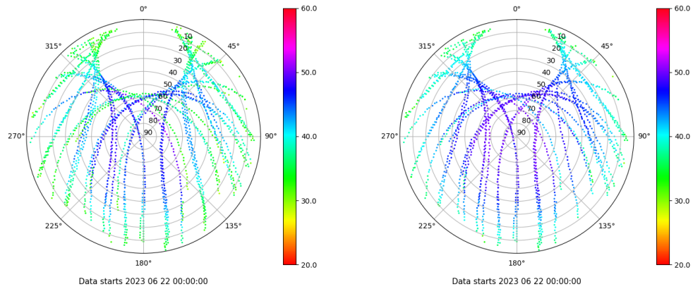
Skyplot for station ZARA. Signal to Noise S1C Data file ZARA00ESP_R_2023173.xtr Skyplot for station ZARA. Signal to Noise S2C Data file ZARA00ESP_R_2023173.xtr
