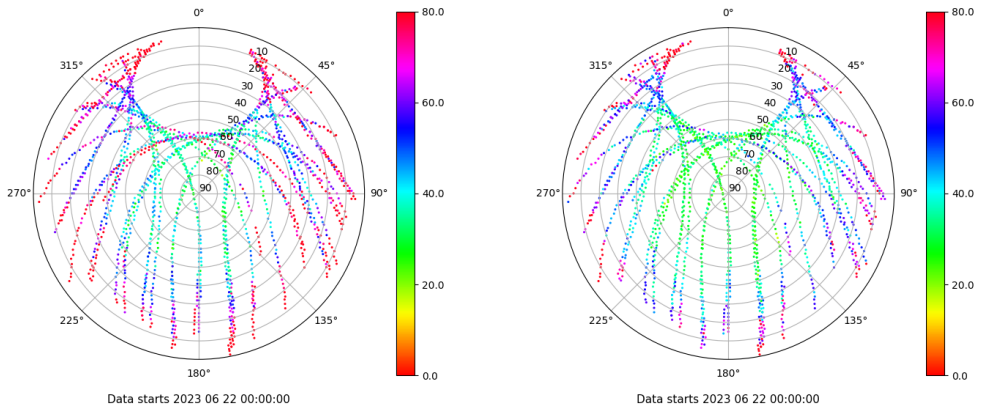
Skyplot for station ZARA. Parameter M1C Data file ZARA00ESP_R_2023173.xtr Skyplot for station ZARA. Parameter M2C Data file ZARA00ESP_R_2023173.xtr
