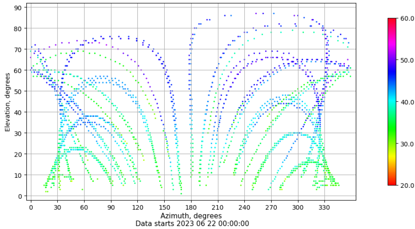
Azimuth-elevation plot for station ZARA. Signal to Noise S1C Data file ZARA00ESP_R_2023173.xtr
