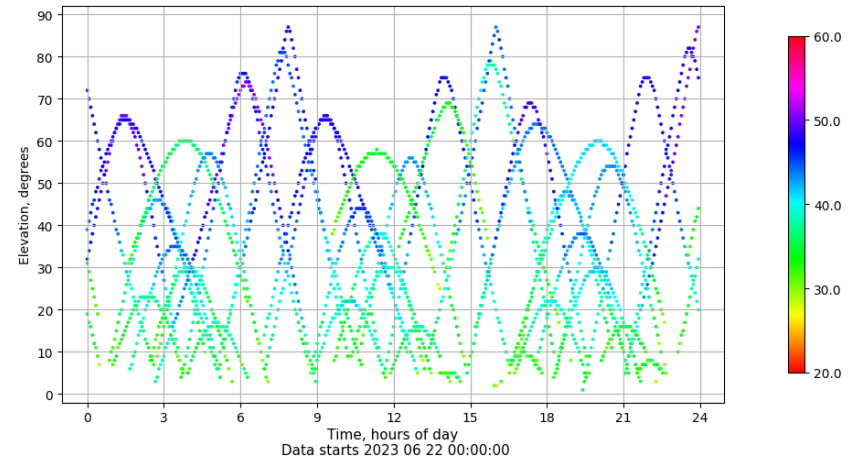
Time-elevation plot for station ZARA. Signal to Noise S1C Data file ZARA00ESP_R_2023173.xtr
