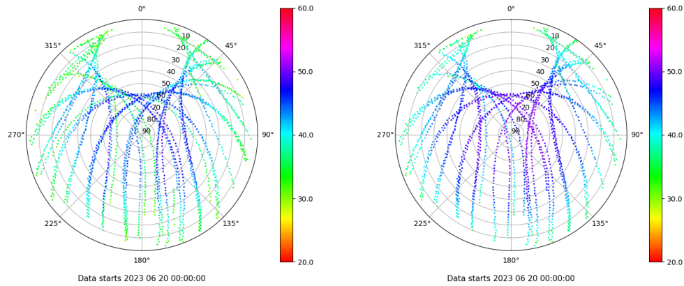
Skyplot for station ZARA. Signal to Noise S1C Data file ZARA00ESP_R_2023171.xtr Skyplot for station ZARA. Signal to Noise S2C Data file ZARA00ESP_R_2023171.xtr
