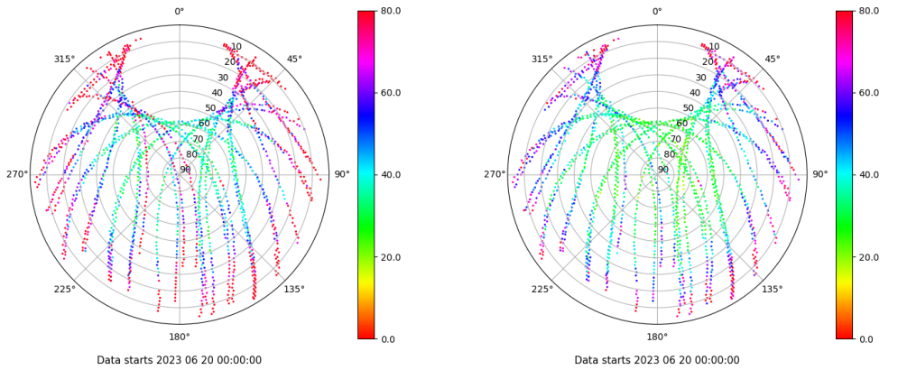
Skyplot for station ZARA. Parameter M1C Data file ZARA00ESP_R_2023171.xtr Skyplot for station ZARA. Parameter M2C Data file ZARA00ESP_R_2023171.xtr
