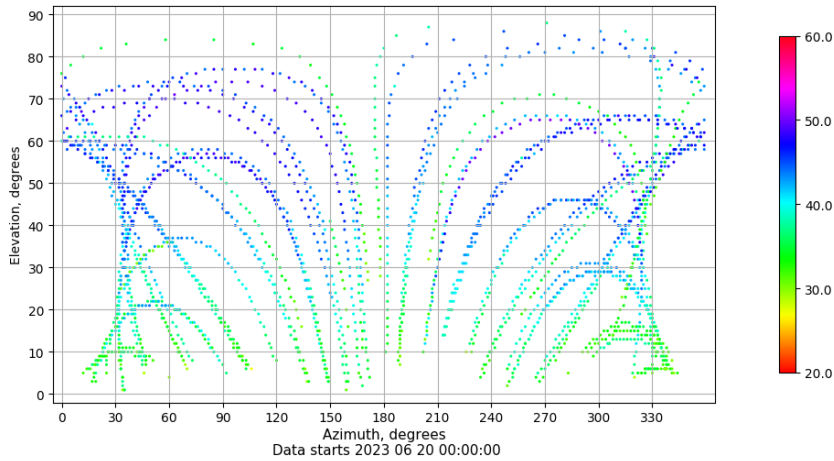
Azimuth-elevation plot for station ZARA. Signal to Noise S1C Data file ZARA00ESP_R_2023171.xtr
