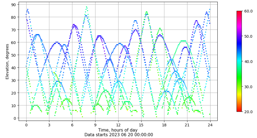
Time-elevation plot for station ZARA. Signal to Noise S1C Data file ZARA00ESP_R_2023171.xtr
