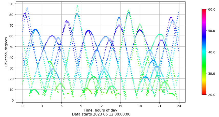
Time-elevation plot for station ZARA. Signal to Noise S1C Data file ZARA00ESP_R_2023163.xtr
