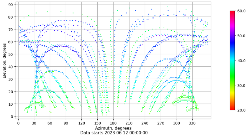
Azimuth-elevation plot for station ZARA. Signal to Noise S1C Data file ZARA00ESP_R_2023163.xtr
