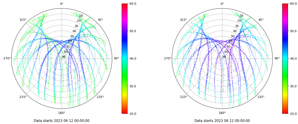
Skyplot for station ZARA. Signal to Noise S1C Data file ZARA00ESP_R_2023163.xtr Skyplot for station ZARA. Signal to Noise S2C Data file ZARA00ESP_R_2023163.xtr
