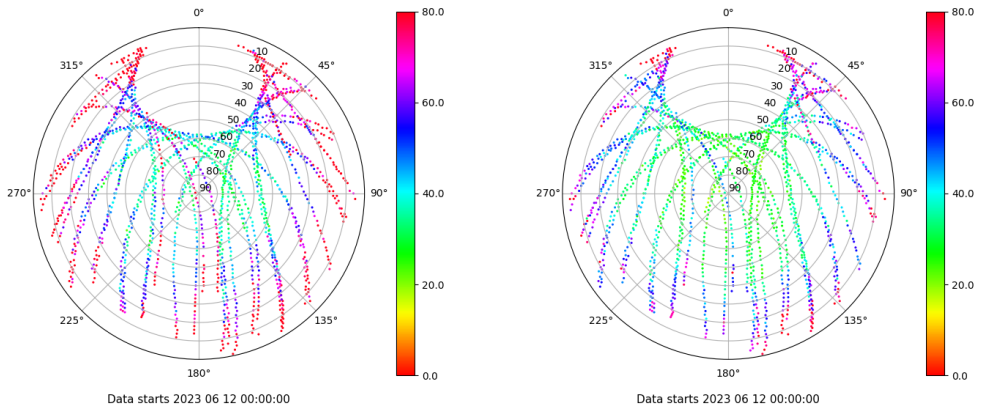
Skyplot for station ZARA. Parameter M1C Data file ZARA00ESP_R_2023163.xtr Skyplot for station ZARA. Parameter M2C Data file ZARA00ESP_R_2023163.xtr
