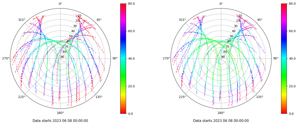
Skyplot for station ZARA. Parameter M1C Data file ZARA00ESP_R_2023159.xtr Skyplot for station ZARA. Parameter M2C Data file ZARA00ESP_R_2023159.xtr
