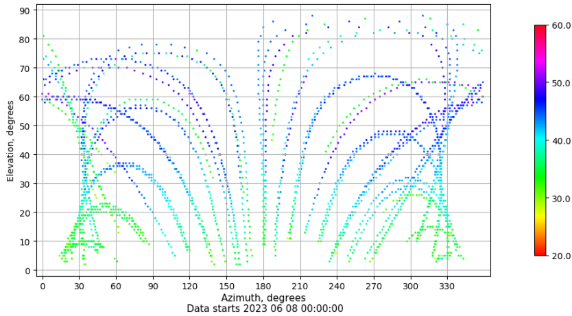
Azimuth-elevation plot for station ZARA. Signal to Noise S1C Data file ZARA00ESP_R_2023159.xtr
