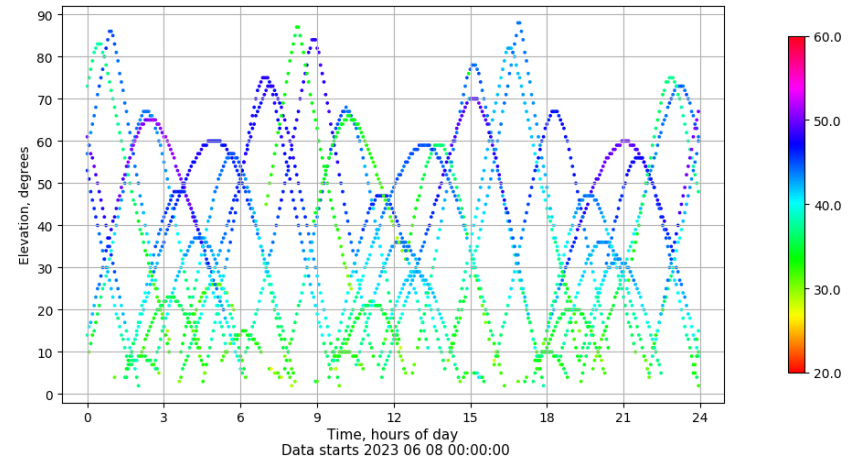
Time-elevation plot for station ZARA. Signal to Noise S1C Data file ZARA00ESP_R_2023159.xtr
