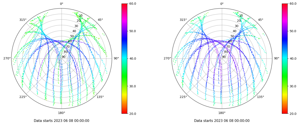
Skyplot for station ZARA. Signal to Noise S1C Data file ZARA00ESP_R_2023159.xtr Skyplot for station ZARA. Signal to Noise S2C Data file ZARA00ESP_R_2023159.xtr
