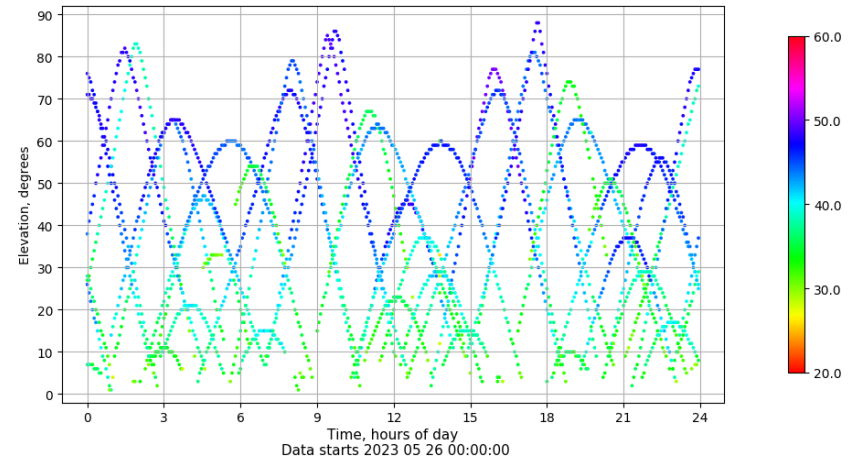
Time-elevation plot for station ZARA. Signal to Noise S1C Data file ZARA00ESP_R_2023146.xtr
