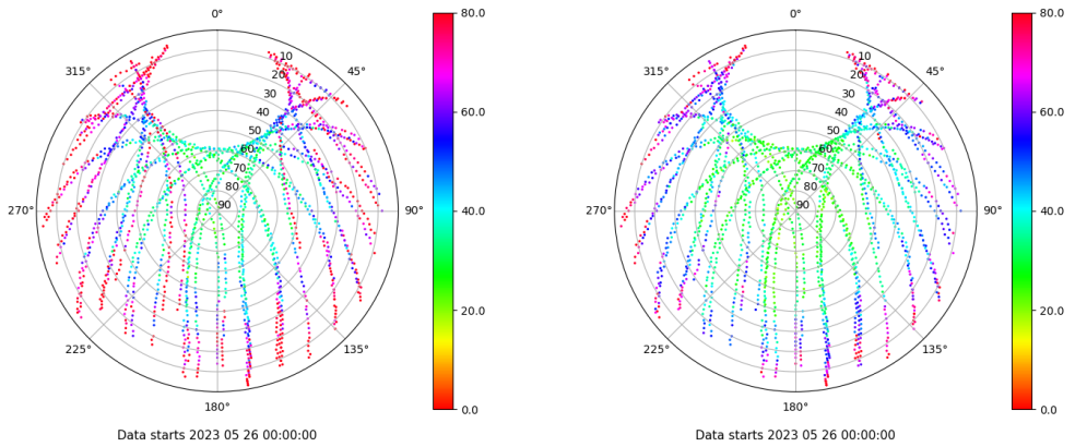
Skyplot for station ZARA. Parameter M1C Data file ZARA00ESP_R_2023146.xtr Skyplot for station ZARA. Parameter M2C Data file ZARA00ESP_R_2023146.xtr
