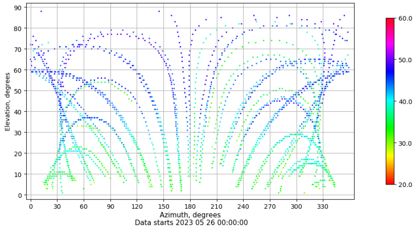
Azimuth-elevation plot for station ZARA. Signal to Noise S1C Data file ZARA00ESP_R_2023146.xtr
