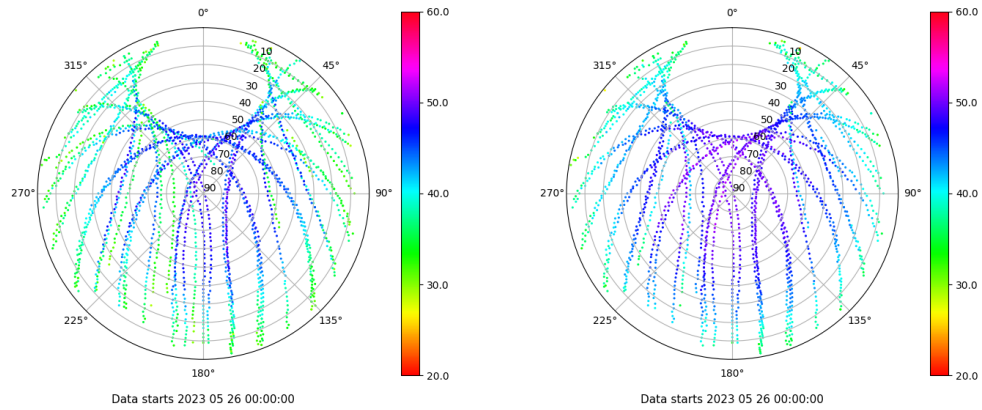
Skyplot for station ZARA. Signal to Noise S1C Data file ZARA00ESP_R_2023146.xtr Skyplot for station ZARA. Signal to Noise S2C Data file ZARA00ESP_R_2023146.xtr
