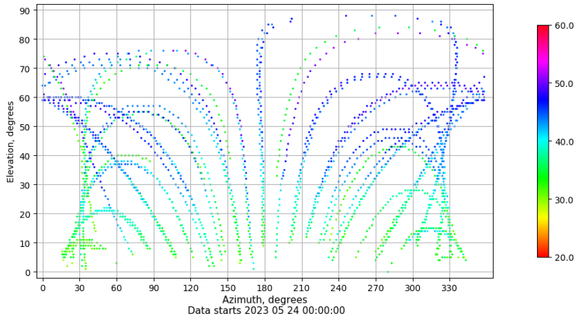
Azimuth-elevation plot for station ZARA. Signal to Noise S1C Data file ZARA00ESP_R_2023144.xtr
