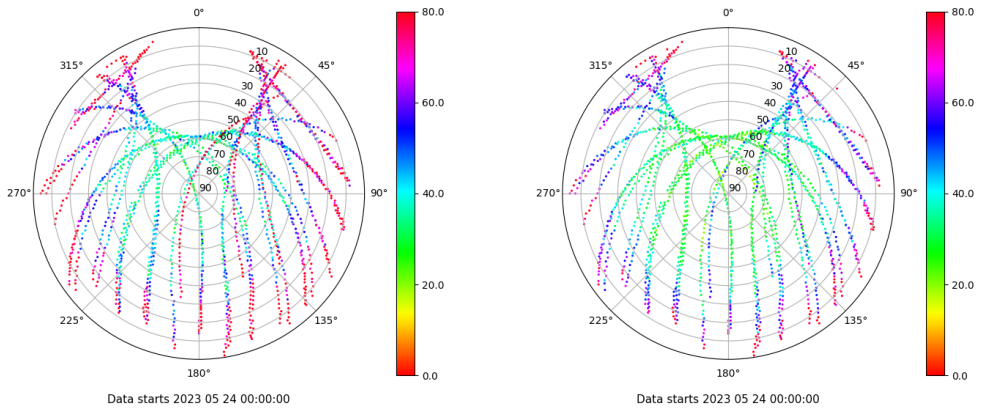
Skyplot for station ZARA. Parameter M1C Data file ZARA00ESP_R_2023144.xtr Skyplot for station ZARA. Parameter M2C Data file ZARA00ESP_R_2023144.xtr
