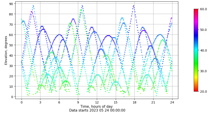
Time-elevation plot for station ZARA. Signal to Noise S1C Data file ZARA00ESP_R_2023144.xtr
