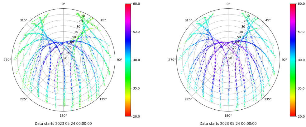
Skyplot for station ZARA. Signal to Noise S1C Data file ZARA00ESP_R_2023144.xtr Skyplot for station ZARA. Signal to Noise S2C Data file ZARA00ESP_R_2023144.xtr
