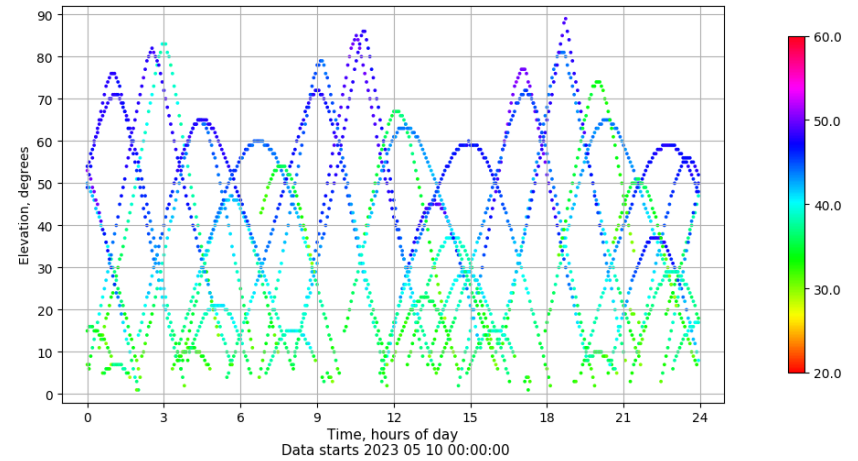
Time-elevation plot for station ZARA. Signal to Noise S1C Data file ZARA00ESP_R_2023130.xtr
