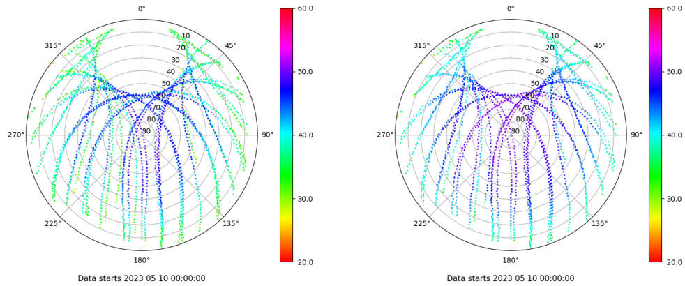
Skyplot for station ZARA. Signal to Noise S1C Data file ZARA00ESP_R_2023130.xtr Skyplot for station ZARA. Signal to Noise S2C Data file ZARA00ESP_R_2023130.xtr
