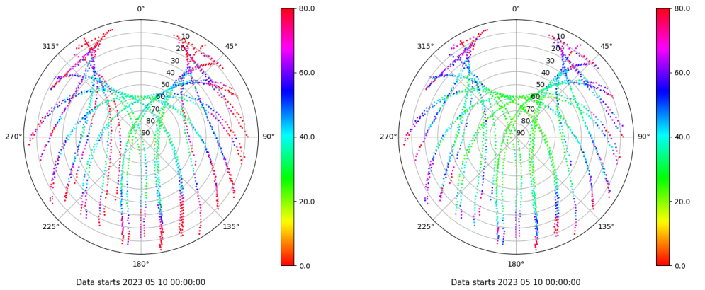
Skyplot for station ZARA. Parameter M1C Data file ZARA00ESP_R_2023130.xtr Skyplot for station ZARA. Parameter M2C Data file ZARA00ESP_R_2023130.xtr
