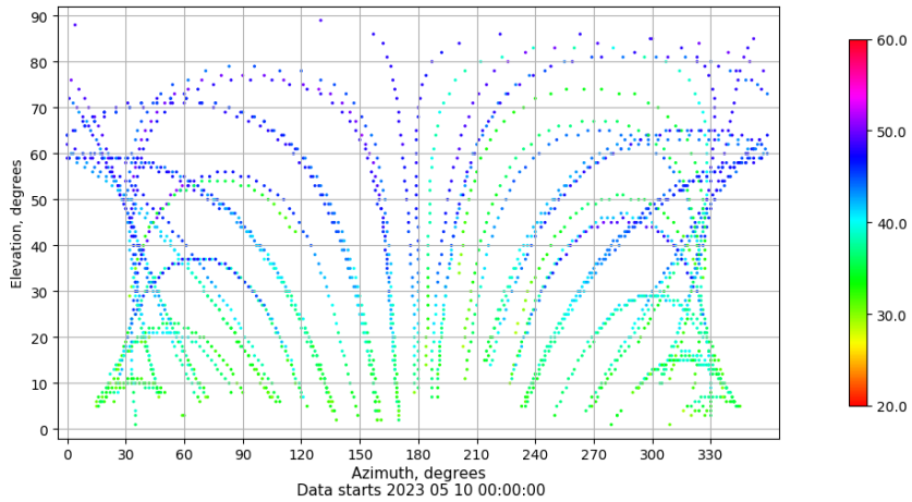
Azimuth-elevation plot for station ZARA. Signal to Noise S1C Data file ZARA00ESP_R_2023130.xtr
