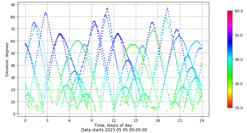
Time-elevation plot for station ZARA. Signal to Noise S1C Data file ZARA00ESP_R_2023125.xtr
