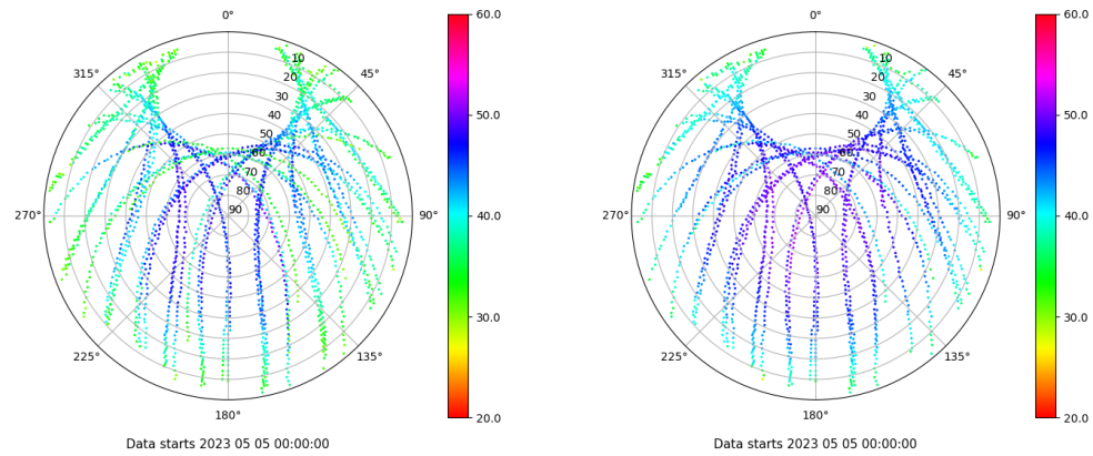
Skyplot for station ZARA. Signal to Noise S1C Data file ZARA00ESP_R_2023125.xtr Skyplot for station ZARA. Signal to Noise S2C Data file ZARA00ESP_R_2023125.xtr
