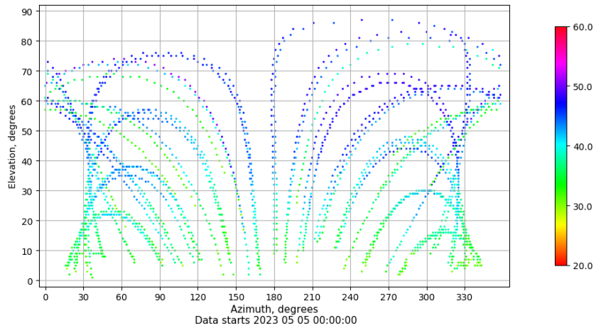
Azimuth-elevation plot for station ZARA. Signal to Noise S1C Data file ZARA00ESP_R_2023125.xtr
