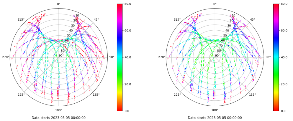
Skyplot for station ZARA. Parameter M1C Data file ZARA00ESP_R_2023125.xtr Skyplot for station ZARA. Parameter M2C Data file ZARA00ESP_R_2023125.xtr
