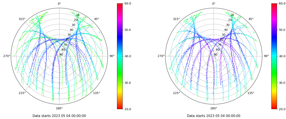
Skyplot for station ZARA. Signal to Noise S1C Data file ZARA00ESP_R_2023124.xtr Skyplot for station ZARA. Signal to Noise S2C Data file ZARA00ESP_R_2023124.xtr
