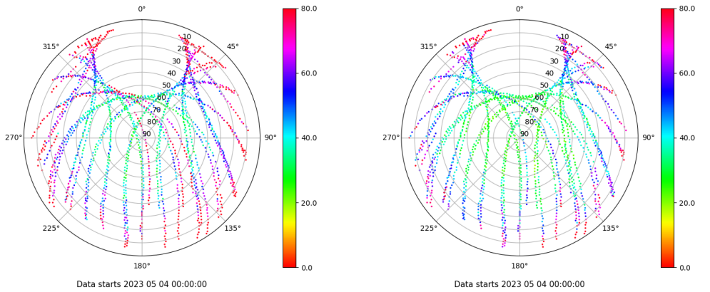
Skyplot for station ZARA. Parameter M1C Data file ZARA00ESP_R_2023124.xtr Skyplot for station ZARA. Parameter M2C Data file ZARA00ESP_R_2023124.xtr
