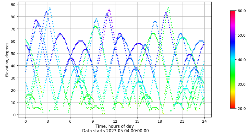
Time-elevation plot for station ZARA. Signal to Noise S1C Data file ZARA00ESP_R_2023124.xtr
