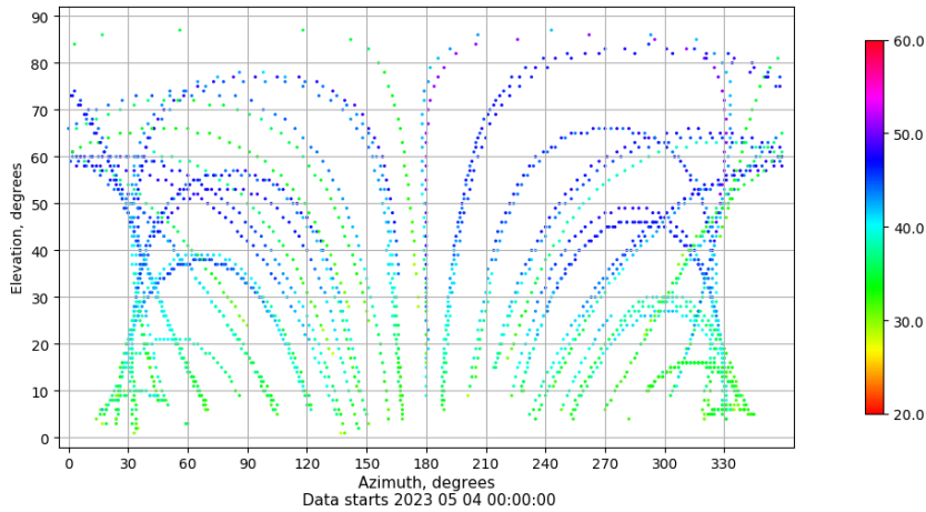
Azimuth-elevation plot for station ZARA. Signal to Noise S1C Data file ZARA00ESP_R_2023124.xtr
