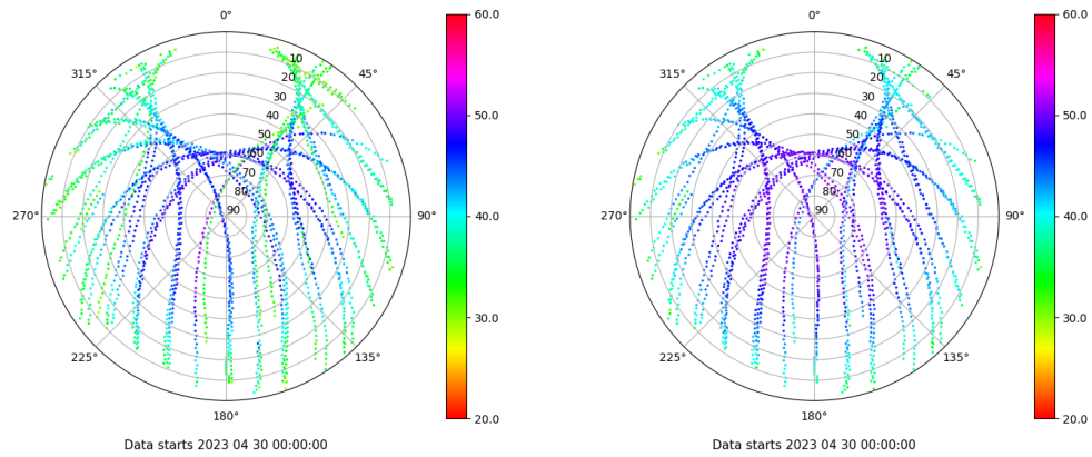
Skyplot for station ZARA. Signal to Noise S1C Data file ZARA00ESP_R_2023120.xtr Skyplot for station ZARA. Signal to Noise S2C Data file ZARA00ESP_R_2023120.xtr
