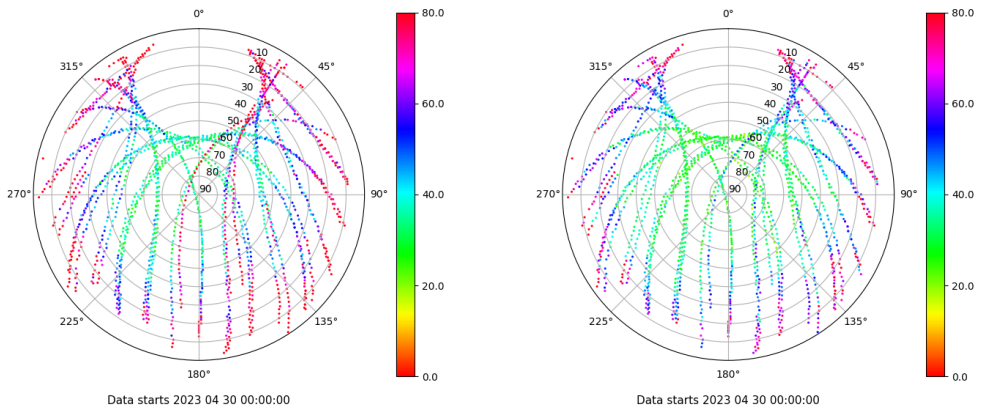
Skyplot for station ZARA. Parameter M1C Data file ZARA00ESP_R_2023120.xtr Skyplot for station ZARA. Parameter M2C Data file ZARA00ESP_R_2023120.xtr
