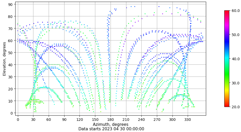
Azimuth-elevation plot for station ZARA. Signal to Noise S1C Data file ZARA00ESP_R_2023120.xtr
