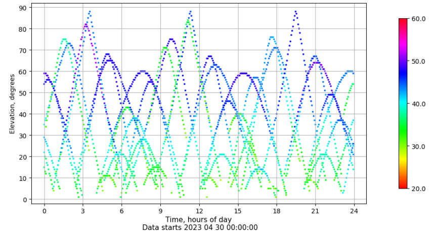
Time-elevation plot for station ZARA. Signal to Noise S1C Data file ZARA00ESP_R_2023120.xtr
