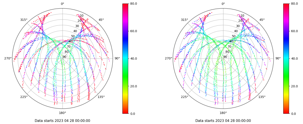
Skyplot for station ZARA. Parameter M1C Data file ZARA00ESP_R_2023118.xtr Skyplot for station ZARA. Parameter M2C Data file ZARA00ESP_R_2023118.xtr
