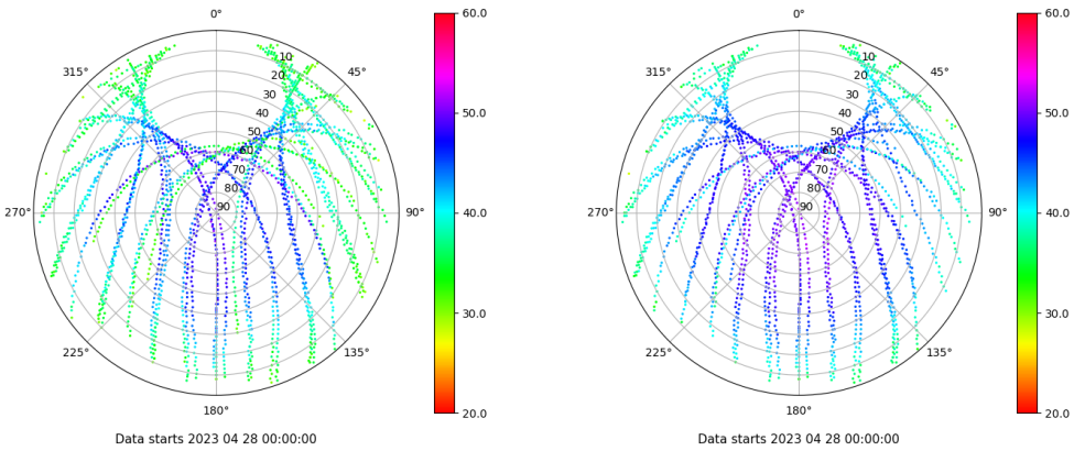
Skyplot for station ZARA. Signal to Noise S1C Data file ZARA00ESP_R_2023118.xtr Skyplot for station ZARA. Signal to Noise S2C Data file ZARA00ESP_R_2023118.xtr
