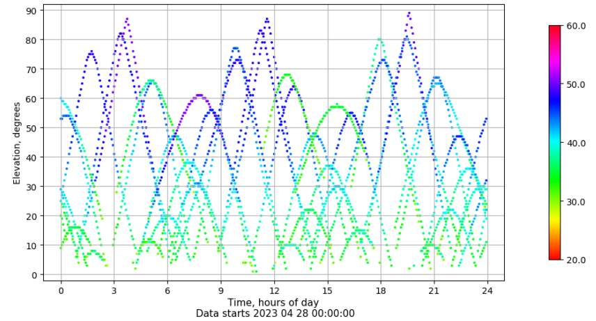
Time-elevation plot for station ZARA. Signal to Noise S1C Data file ZARA00ESP_R_2023118.xtr
