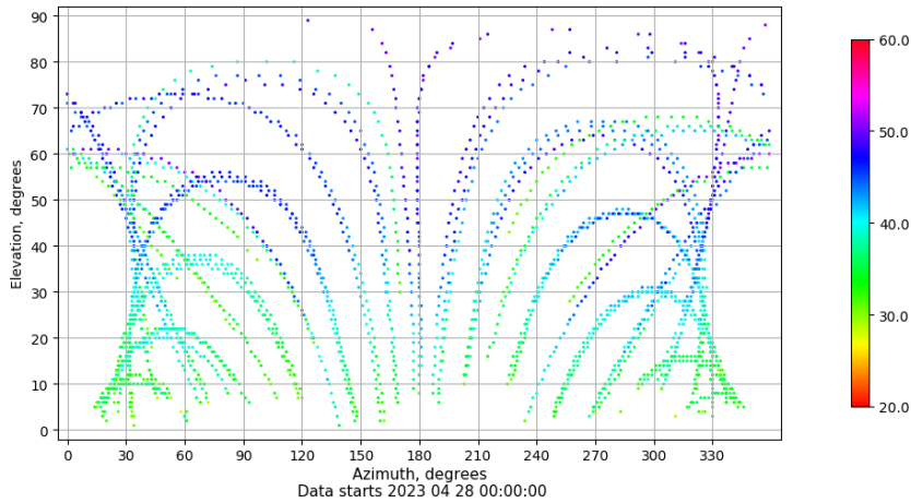
Azimuth-elevation plot for station ZARA. Signal to Noise S1C Data file ZARA00ESP_R_2023118.xtr
