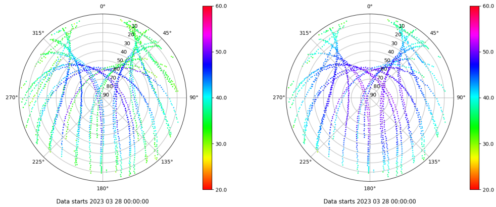
Skyplot for station ZARA. Signal to Noise S1C Data file ZARA00ESP_R_2023087.xtr Skyplot for station ZARA. Signal to Noise S2C Data file ZARA00ESP_R_2023087.xtr
