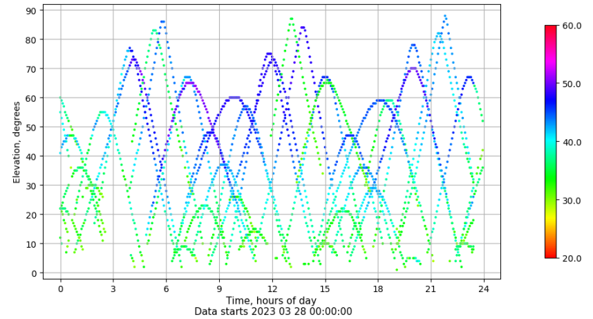
Time-elevation plot for station ZARA. Signal to Noise S1C Data file ZARA00ESP_R_2023087.xtr
