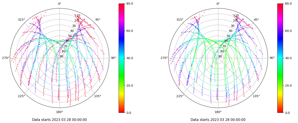
Skyplot for station ZARA. Parameter M1C Data file ZARA00ESP_R_2023087.xtr Skyplot for station ZARA. Parameter M2C Data file ZARA00ESP_R_2023087.xtr
