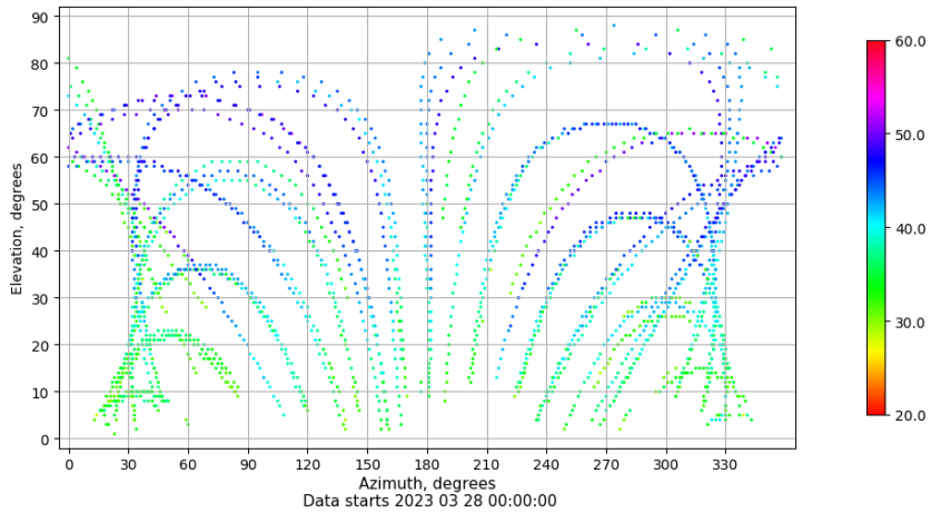
Azimuth-elevation plot for station ZARA. Signal to Noise S1C Data file ZARA00ESP_R_2023087.xtr
