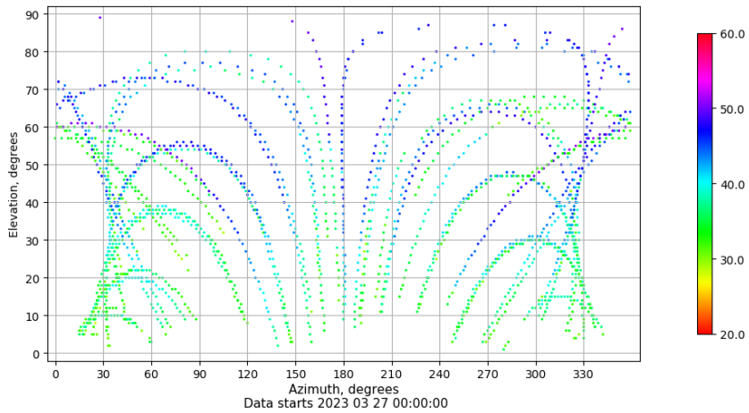
Azimuth-elevation plot for station ZARA. Signal to Noise S1C Data file ZARA00ESP_R_2023086.xtr
