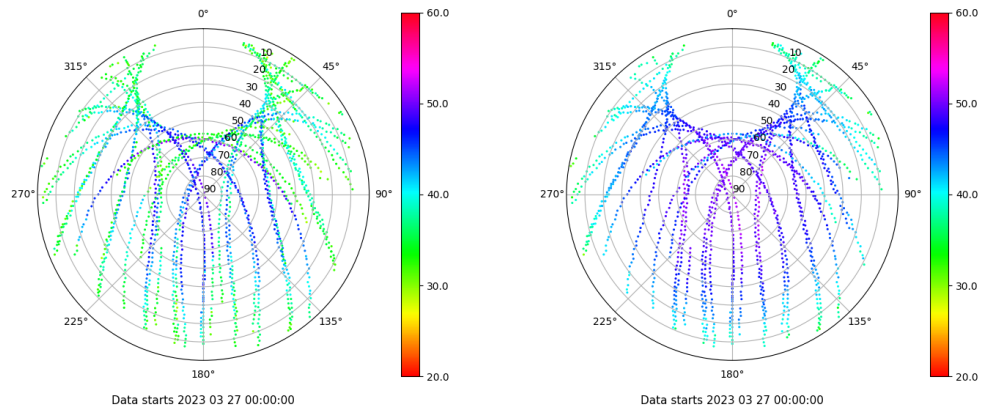
Skyplot for station ZARA. Signal to Noise S1C Data file ZARA00ESP_R_2023086.xtr Skyplot for station ZARA. Signal to Noise S2C Data file ZARA00ESP_R_2023086.xtr
