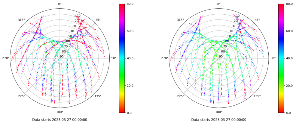
Skyplot for station ZARA. Parameter M1C Data file ZARA00ESP_R_2023086.xtr Skyplot for station ZARA. Parameter M2C Data file ZARA00ESP_R_2023086.xtr
