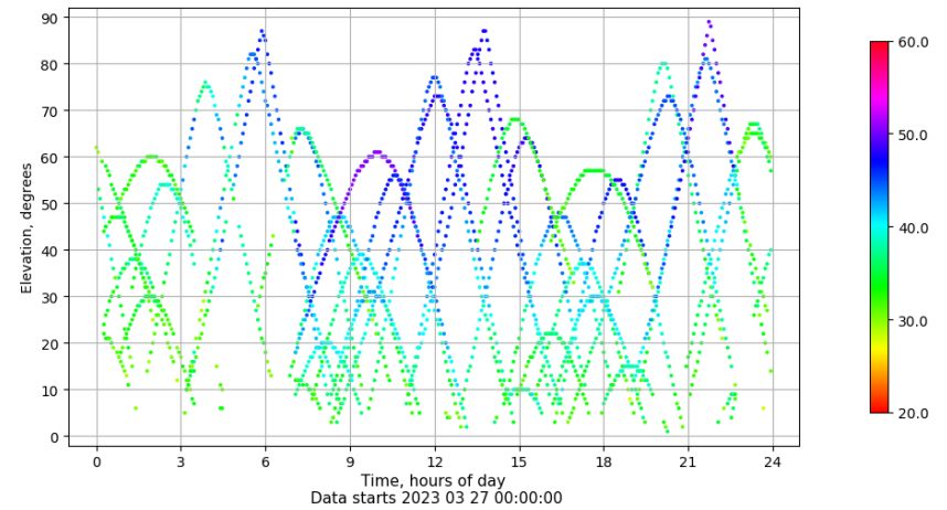
Time-elevation plot for station ZARA. Signal to Noise S1C Data file ZARA00ESP_R_2023086.xtr
