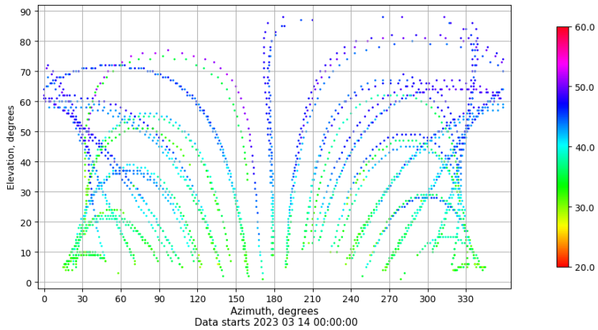
Azimuth-elevation plot for station ZARA. Signal to Noise S1C Data file ZARA00ESP_R_2023073.xtr
