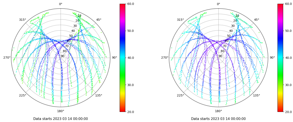
Skyplot for station ZARA. Signal to Noise S1C Data file ZARA00ESP_R_2023073.xtr Skyplot for station ZARA. Signal to Noise S2C Data file ZARA00ESP_R_2023073.xtr
