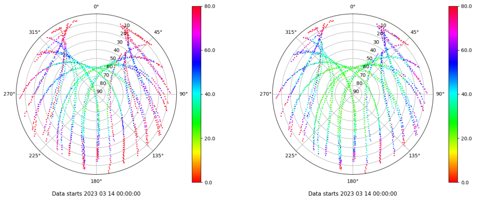
Skyplot for station ZARA. Parameter M1C Data file ZARA00ESP_R_2023073.xtr Skyplot for station ZARA. Parameter M2C Data file ZARA00ESP_R_2023073.xtr
