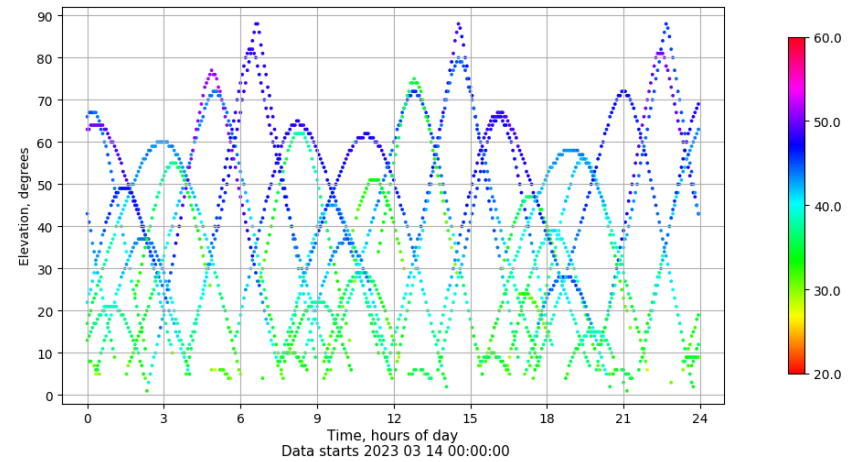
Time-elevation plot for station ZARA. Signal to Noise S1C Data file ZARA00ESP_R_2023073.xtr
