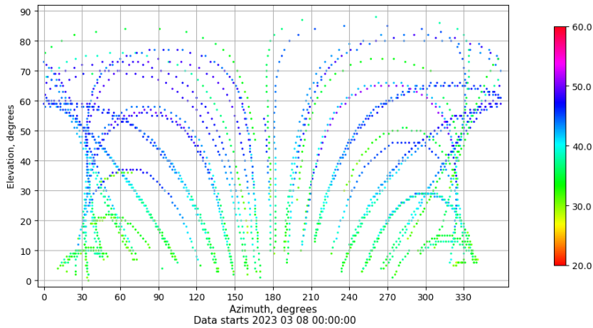
Azimuth-elevation plot for station ZARA. Signal to Noise S1C Data file ZARA00ESP_R_2023067.xtr
