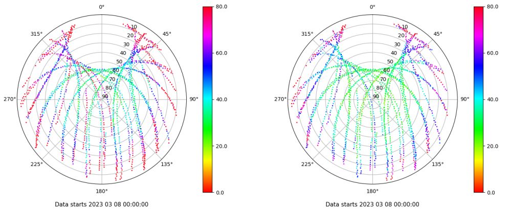
Skyplot for station ZARA. Parameter M1C Data file ZARA00ESP_R_2023067.xtr Skyplot for station ZARA. Parameter M2C Data file ZARA00ESP_R_2023067.xtr
