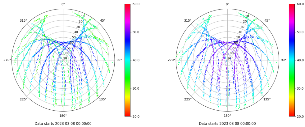
Skyplot for station ZARA. Signal to Noise S1C Data file ZARA00ESP_R_2023067.xtr Skyplot for station ZARA. Signal to Noise S2C Data file ZARA00ESP_R_2023067.xtr
