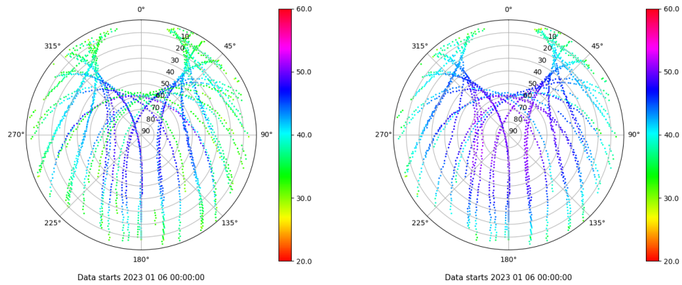
Skyplot for station ZARA. Signal to Noise S1C Data file ZARA00ESP_R_2023006.xtr Skyplot for station ZARA. Signal to Noise S2C Data file ZARA00ESP_R_2023006.xtr
