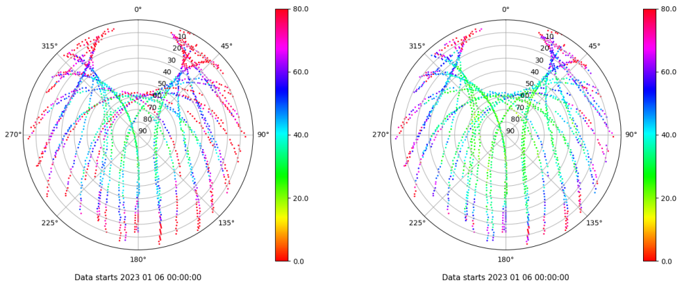
Skyplot for station ZARA. Parameter M1C Data file ZARA00ESP_R_2023006.xtr Skyplot for station ZARA. Parameter M2C Data file ZARA00ESP_R_2023006.xtr
