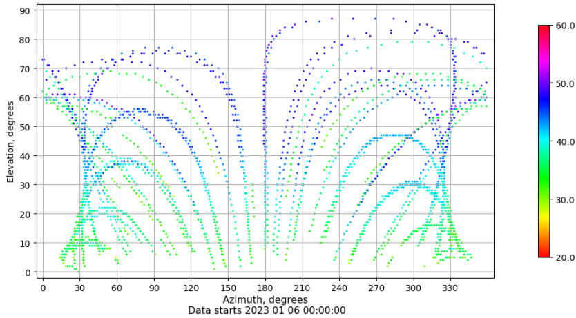
Azimuth-elevation plot for station ZARA. Signal to Noise S1C Data file ZARA00ESP_R_2023006.xtr
