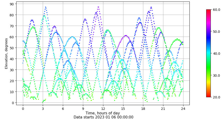
Time-elevation plot for station ZARA. Signal to Noise S1C Data file ZARA00ESP_R_2023006.xtr
