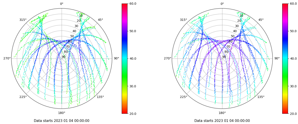
Skyplot for station ZARA. Signal to Noise S1C Data file ZARA00ESP_R_2023004.xtr Skyplot for station ZARA. Signal to Noise S2C Data file ZARA00ESP_R_2023004.xtr
