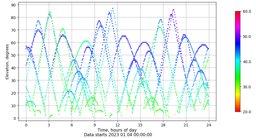
Time-elevation plot for station ZARA. Signal to Noise S1C Data file ZARA00ESP_R_2023004.xtr
