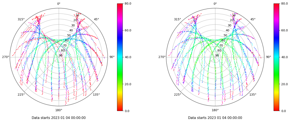
Skyplot for station ZARA. Parameter M1C Data file ZARA00ESP_R_2023004.xtr Skyplot for station ZARA. Parameter M2C Data file ZARA00ESP_R_2023004.xtr
