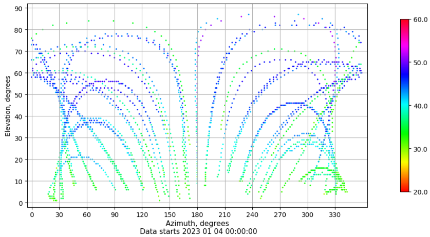
Azimuth-elevation plot for station ZARA. Signal to Noise S1C Data file ZARA00ESP_R_2023004.xtr
