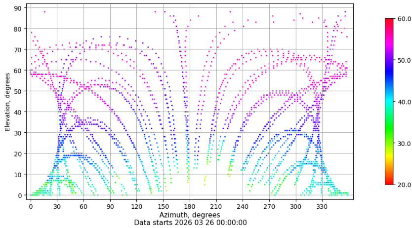
Azimuth-elevation plot for station YEBE. Signal to Noise S1C Data file YEBE00ESP_R_2026085.xtr
