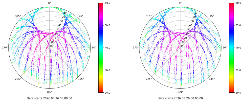
Skyplot for station YEBE. Signal to Noise S1C Data file YEBE00ESP_R_2026085.xtr Skyplot for station YEBE. Signal to Noise S2C Data file YEBE00ESP_R_2026085.xtr
