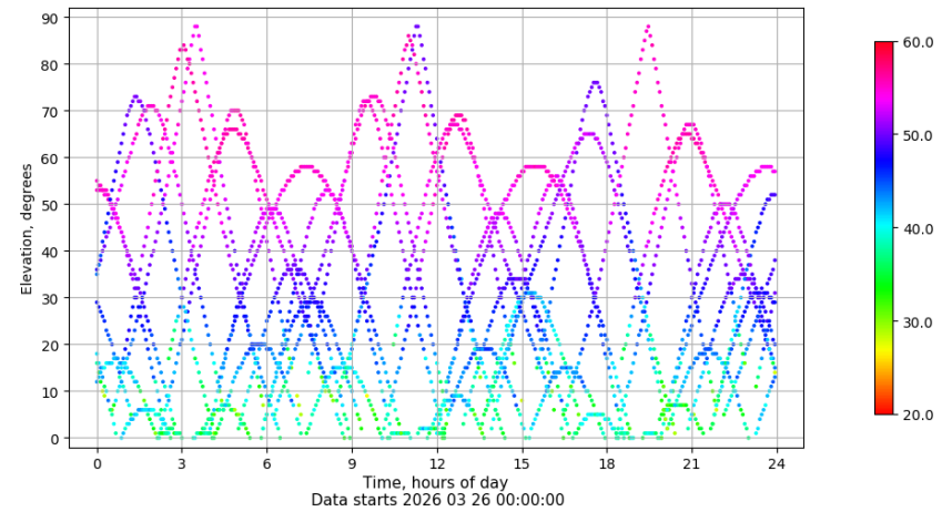
Time-elevation plot for station YEBE. Signal to Noise S1C Data file YEBE00ESP_R_2026085.xtr
