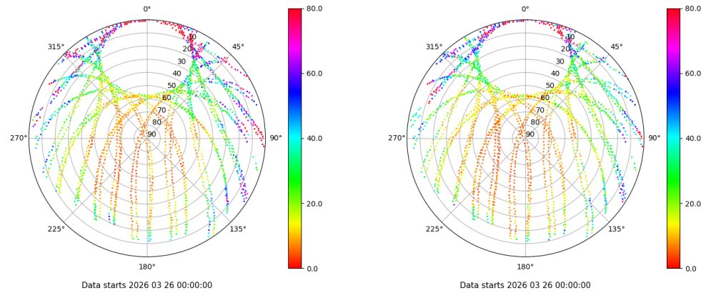
Skyplot for station YEBE. Parameter M1C Data file YEBE00ESP_R_2026085.xtr Skyplot for station YEBE. Parameter M2C Data file YEBE00ESP_R_2026085.xtr
