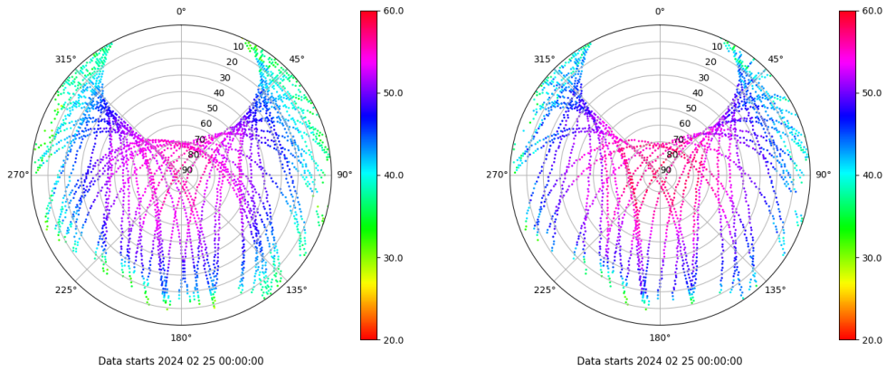
Skyplot for station YEBE. Signal to Noise S1C Data file YEBE00ESP_R_2024056.xtr Skyplot for station YEBE. Signal to Noise S2S Data file YEBE00ESP_R_2024056.xtr
