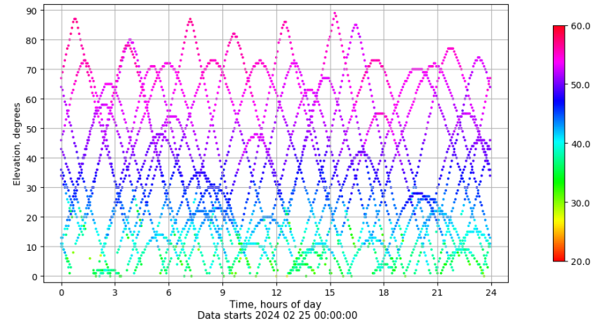
Time-elevation plot for station YEBE. Signal to Noise S1C Data file YEBE00ESP_R_2024056.xtr
