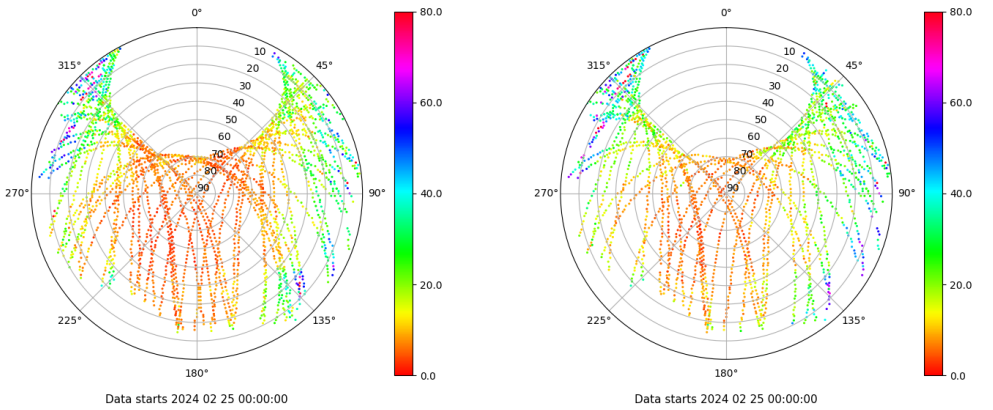
Skyplot for station YEBE. Parameter M1C Data file YEBE00ESP_R_2024056.xtr Skyplot for station YEBE. Parameter M2S Data file YEBE00ESP_R_2024056.xtr
