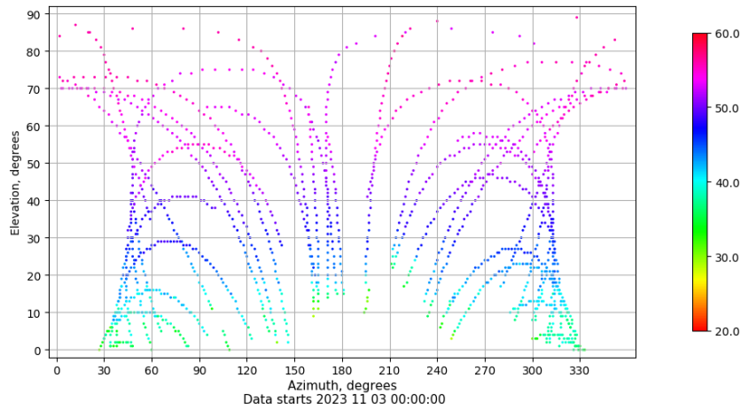
Azimuth-elevation plot for station YEBE. Signal to Noise S1C Data file YEBE00ESP_R_2023307.xtr
