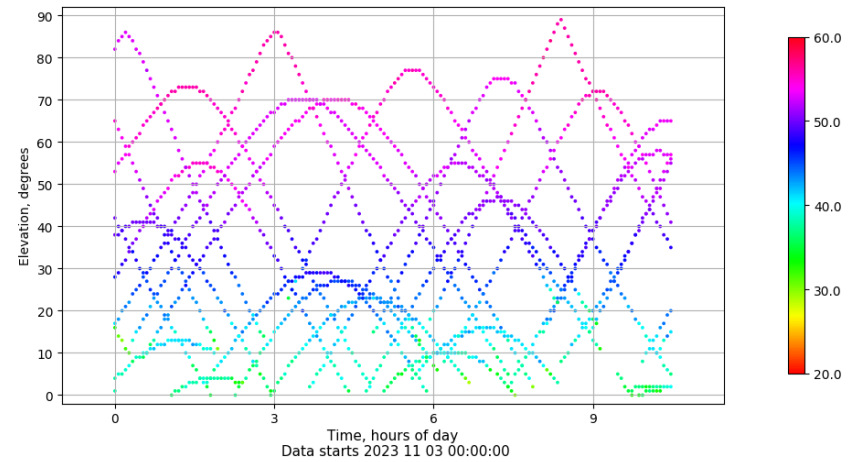
Time-elevation plot for station YEBE. Signal to Noise S1C Data file YEBE00ESP_R_2023307.xtr
