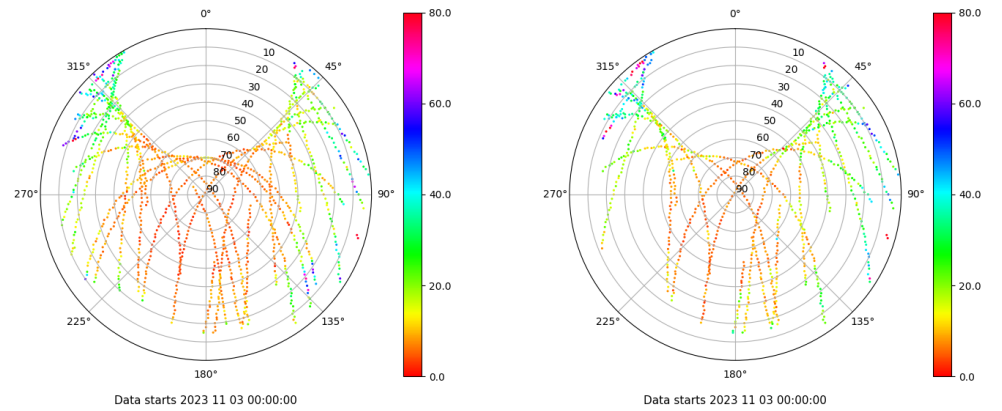
Skyplot for station YEBE. Parameter M1C Data file YEBE00ESP_R_2023307.xtr Skyplot for station YEBE. Parameter M2S Data file YEBE00ESP_R_2023307.xtr
