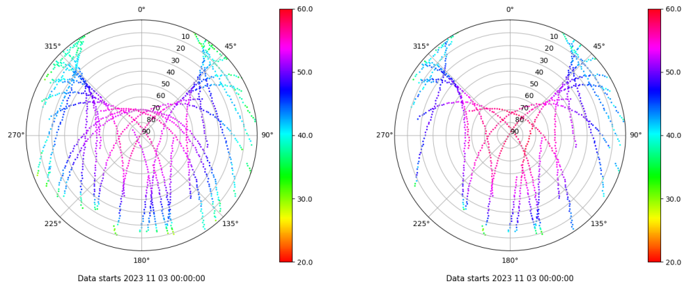
Skyplot for station YEBE. Signal to Noise S1C Data file YEBE00ESP_R_2023307.xtr Skyplot for station YEBE. Signal to Noise S2S Data file YEBE00ESP_R_2023307.xtr
