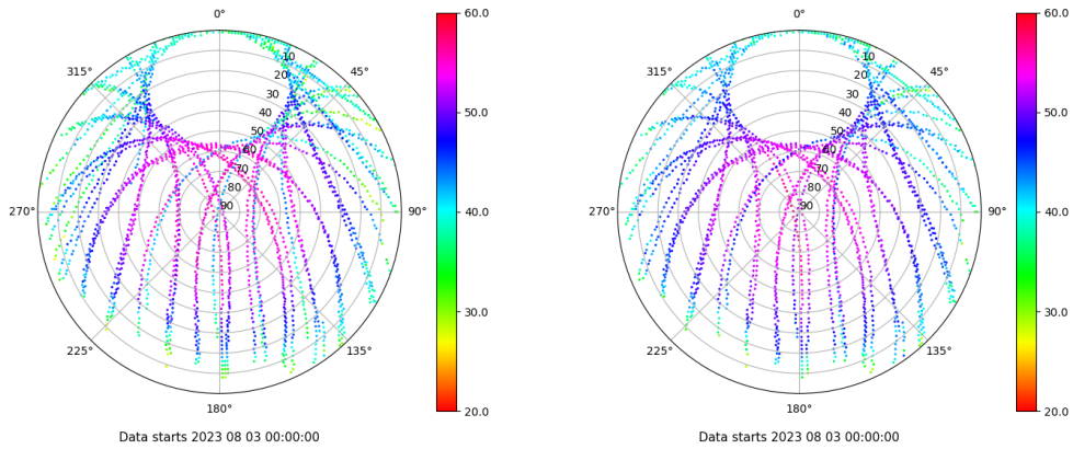
Skyplot for station YEBE. Signal to Noise S1C Data file YEBE00ESP_R_2023215.xtr Skyplot for station YEBE. Signal to Noise S2C Data file YEBE00ESP_R_2023215.xtr
