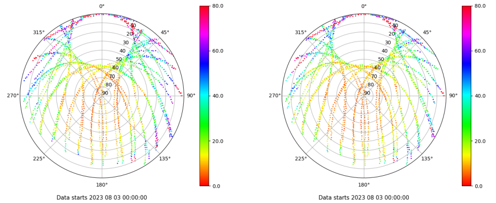
Skyplot for station YEBE. Parameter M1C Data file YEBE00ESP_R_2023215.xtr Skyplot for station YEBE. Parameter M2C Data file YEBE00ESP_R_2023215.xtr
