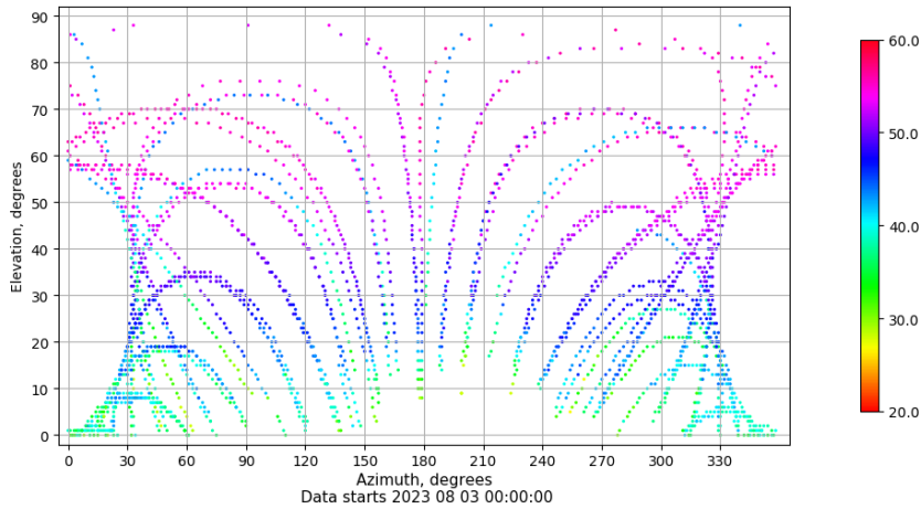
Azimuth-elevation plot for station YEBE. Signal to Noise S1C Data file YEBE00ESP_R_2023215.xtr
