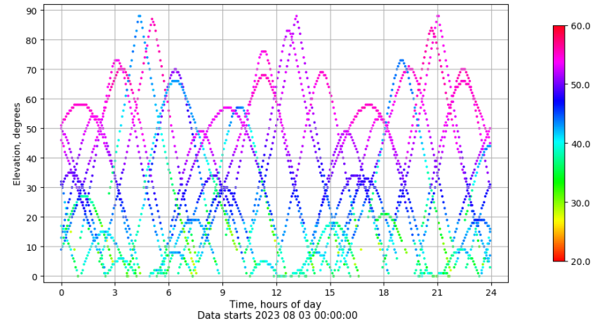
Time-elevation plot for station YEBE. Signal to Noise S1C Data file YEBE00ESP_R_2023215.xtr
