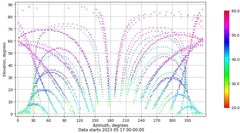
Azimuth-elevation plot for station YEBE. Signal to Noise S1C Data file YEBE00ESP_R_2023137.xtr
