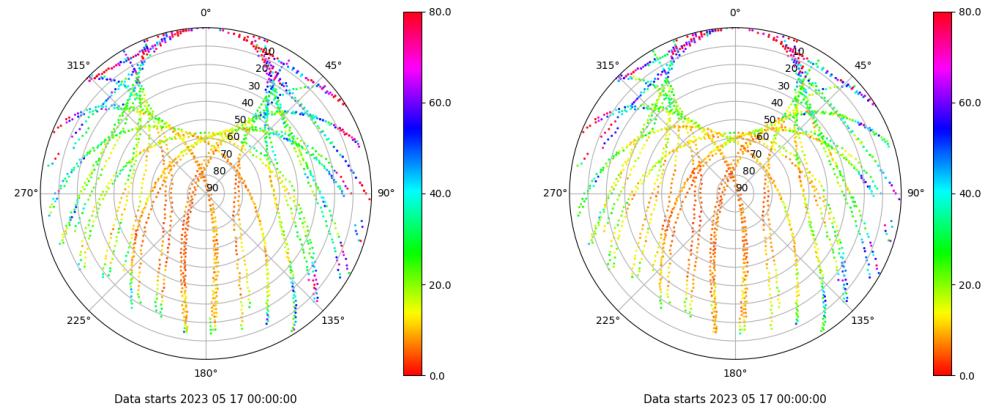
Skyplot for station YEBE. Parameter M1C Data file YEBE00ESP_R_2023137.xtr Skyplot for station YEBE. Parameter M2C Data file YEBE00ESP_R_2023137.xtr
