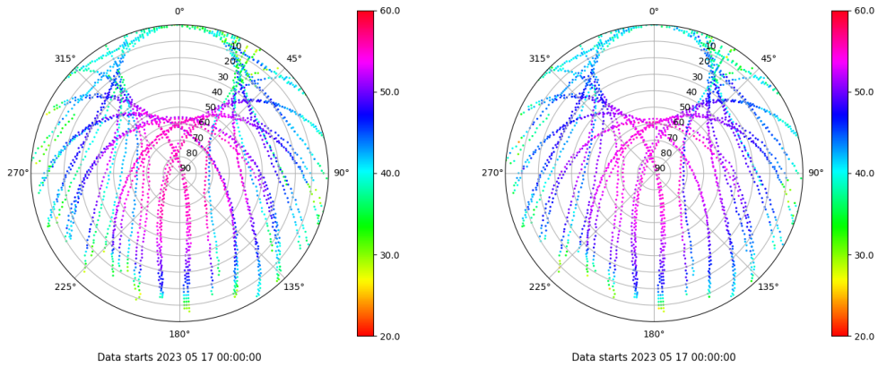
Skyplot for station YEBE. Signal to Noise S1C Data file YEBE00ESP_R_2023137.xtr Skyplot for station YEBE. Signal to Noise S2C Data file YEBE00ESP_R_2023137.xtr
