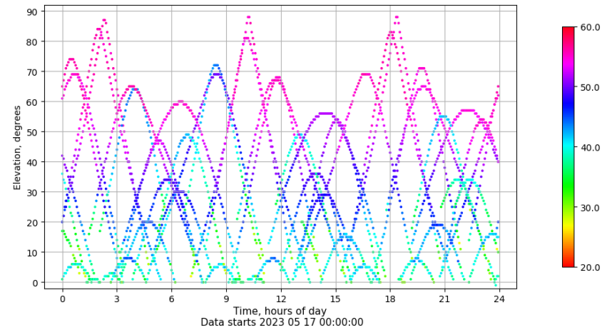
Time-elevation plot for station YEBE. Signal to Noise S1C Data file YEBE00ESP_R_2023137.xtr
