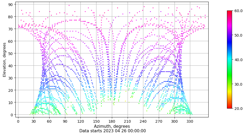
Azimuth-elevation plot for station YEBE. Signal to Noise S1C Data file YEBE00ESP_R_2023116.xtr
