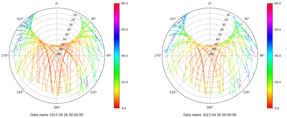
Skyplot for station YEBE. Parameter M1C Data file YEBE00ESP_R_2023116.xtr Skyplot for station YEBE. Parameter M2S Data file YEBE00ESP_R_2023116.xtr
