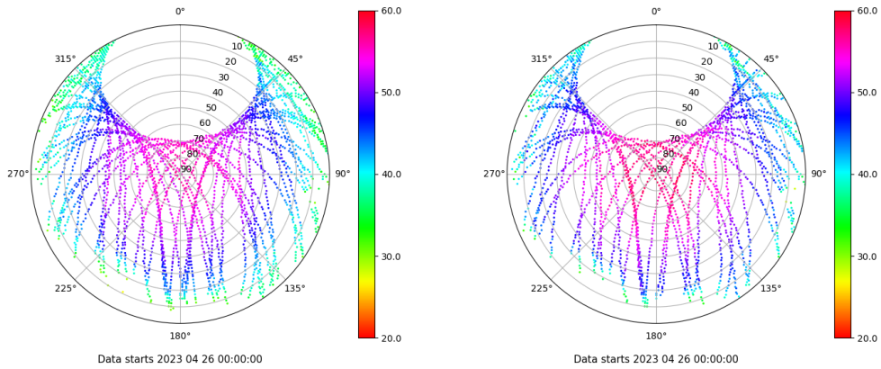
Skyplot for station YEBE. Signal to Noise S1C Data file YEBE00ESP_R_2023116.xtr Skyplot for station YEBE. Signal to Noise S2S Data file YEBE00ESP_R_2023116.xtr
