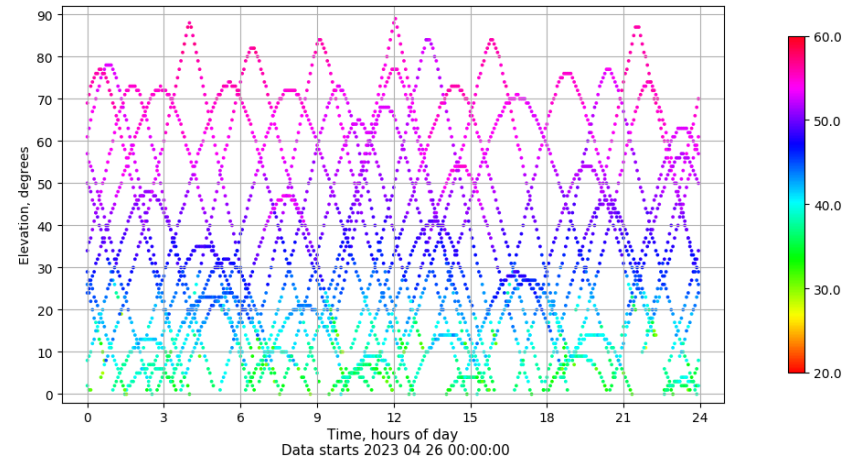
Time-elevation plot for station YEBE. Signal to Noise S1C Data file YEBE00ESP_R_2023116.xtr
