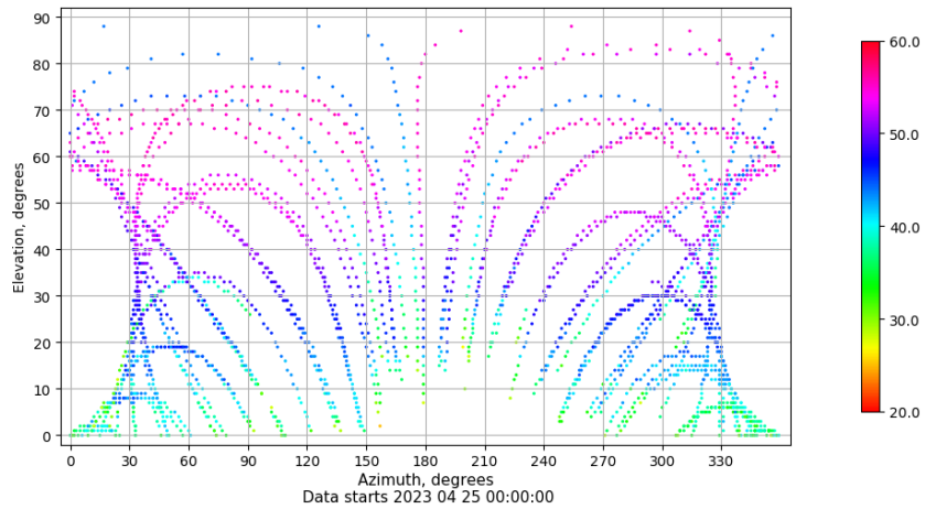
Azimuth-elevation plot for station YEBE. Signal to Noise S1C Data file YEBE00ESP_R_2023115.xtr
