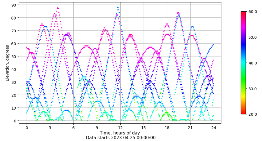
Time-elevation plot for station YEBE. Signal to Noise S1C Data file YEBE00ESP_R_2023115.xtr
