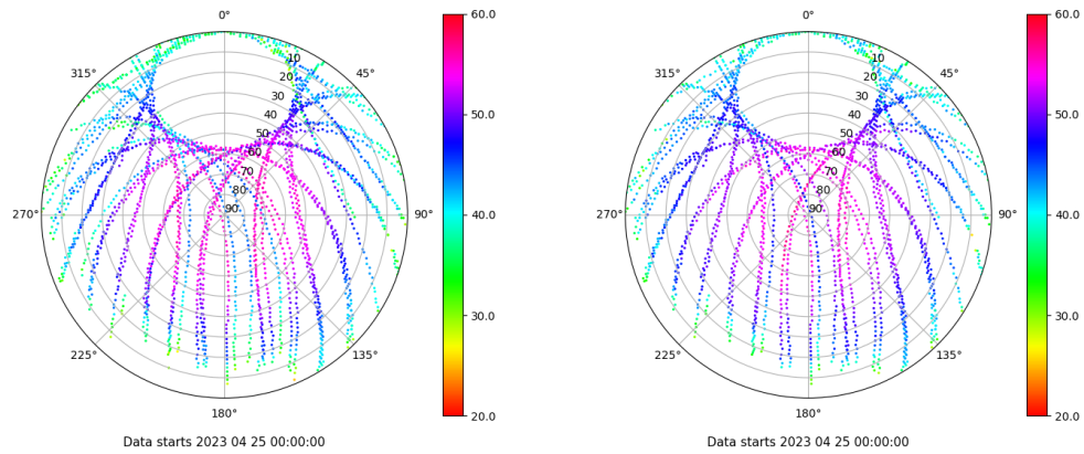
Skyplot for station YEBE. Signal to Noise S1C Data file YEBE00ESP_R_2023115.xtr Skyplot for station YEBE. Signal to Noise S2C Data file YEBE00ESP_R_2023115.xtr
