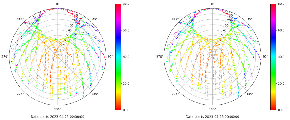
Skyplot for station YEBE. Parameter M1C Data file YEBE00ESP_R_2023115.xtr Skyplot for station YEBE. Parameter M2C Data file YEBE00ESP_R_2023115.xtr
