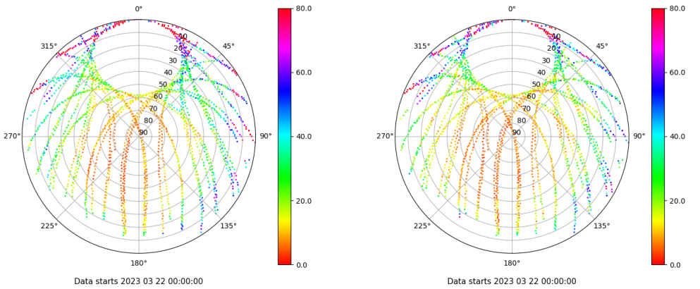
Skyplot for station YEBE. Parameter M1C Data file YEBE00ESP_R_2023081.xtr Skyplot for station YEBE. Parameter M2C Data file YEBE00ESP_R_2023081.xtr
