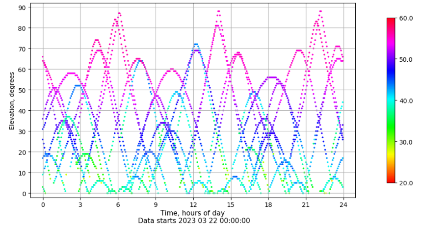
Time-elevation plot for station YEBE. Signal to Noise S1C Data file YEBE00ESP_R_2023081.xtr
