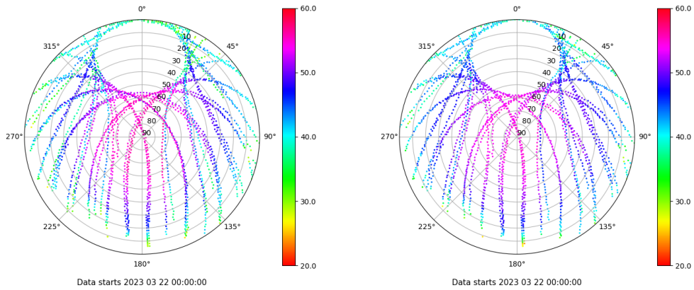
Skyplot for station YEBE. Signal to Noise S1C Data file YEBE00ESP_R_2023081.xtr Skyplot for station YEBE. Signal to Noise S2C Data file YEBE00ESP_R_2023081.xtr
