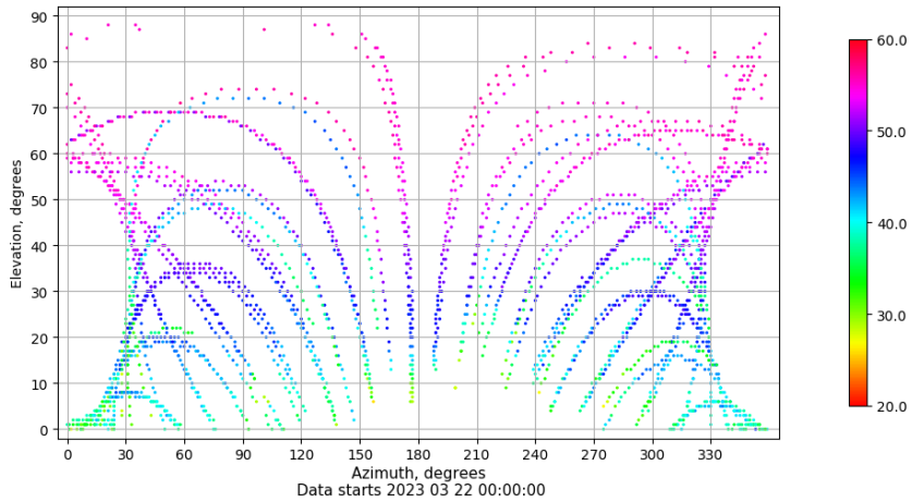
Azimuth-elevation plot for station YEBE. Signal to Noise S1C Data file YEBE00ESP_R_2023081.xtr
