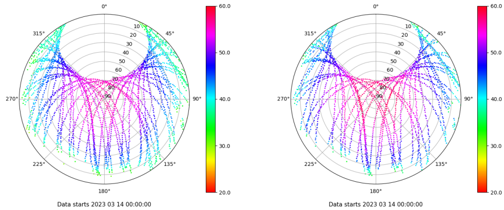
Skyplot for station YEBE. Signal to Noise S1C Data file YEBE00ESP_R_2023073.xtr Skyplot for station YEBE. Signal to Noise S2S Data file YEBE00ESP_R_2023073.xtr
