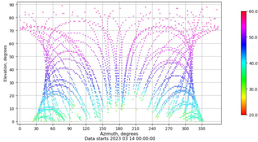
Azimuth-elevation plot for station YEBE. Signal to Noise S1C Data file YEBE00ESP_R_2023073.xtr
