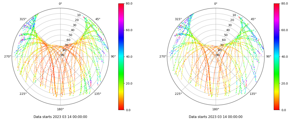
Skyplot for station YEBE. Parameter M1C Data file YEBE00ESP_R_2023073.xtr Skyplot for station YEBE. Parameter M2S Data file YEBE00ESP_R_2023073.xtr
