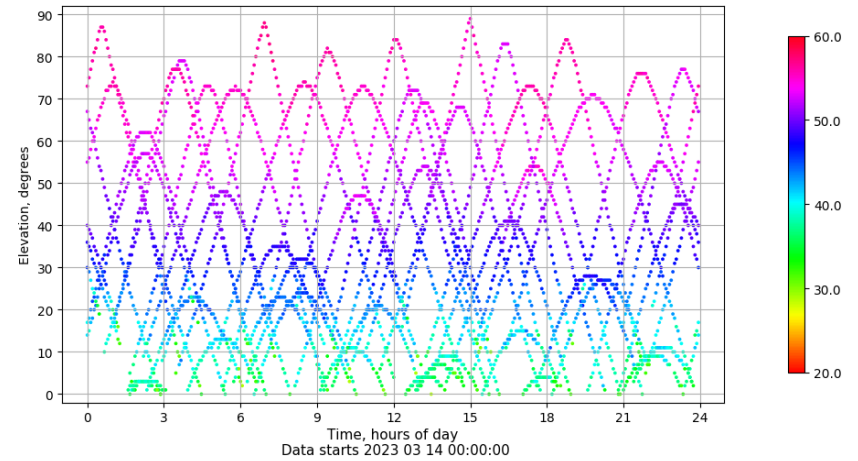
Time-elevation plot for station YEBE. Signal to Noise S1C Data file YEBE00ESP_R_2023073.xtr
