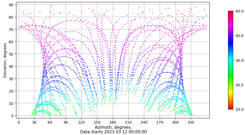
Azimuth-elevation plot for station YEBE. Signal to Noise S1C Data file YEBE00ESP_R_2023071.xtr
