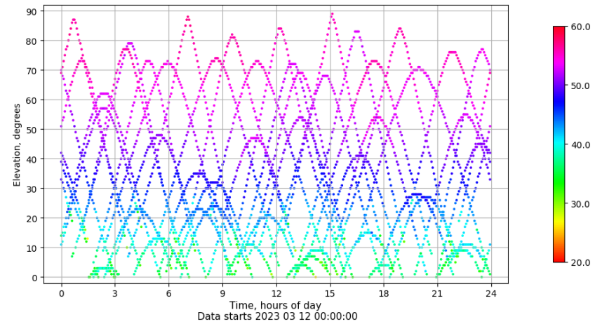
Time-elevation plot for station YEBE. Signal to Noise S1C Data file YEBE00ESP_R_2023071.xtr
