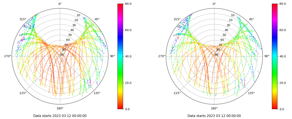
Skyplot for station YEBE. Parameter M1C Data file YEBE00ESP_R_2023071.xtr Skyplot for station YEBE. Parameter M2S Data file YEBE00ESP_R_2023071.xtr
