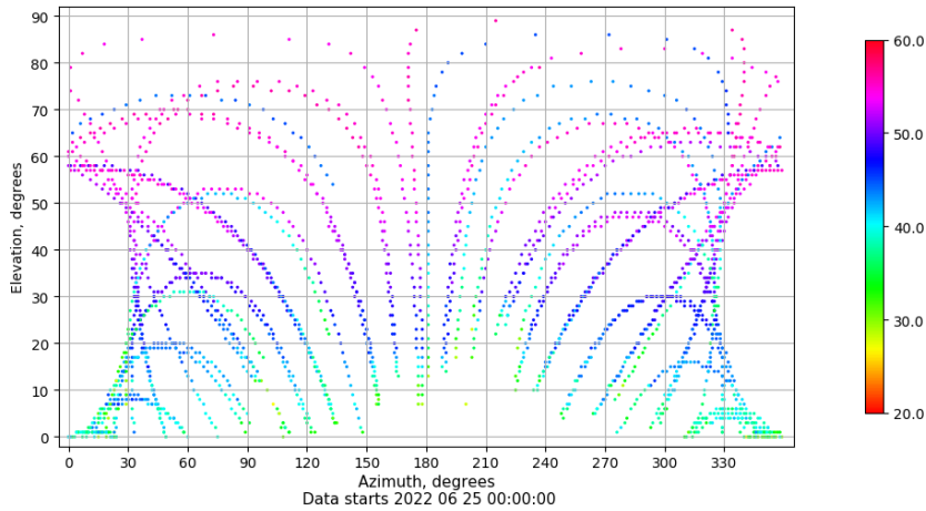
Azimuth-elevation plot for station YEBE. Signal to Noise S1C Data file YEBE00ESP_R_2022176.xtr
