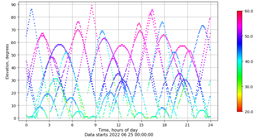
Time-elevation plot for station YEBE. Signal to Noise S1C Data file YEBE00ESP_R_2022176.xtr
