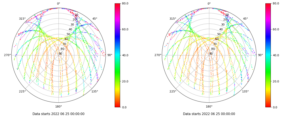
Skyplot for station YEBE. Parameter M1C Data file YEBE00ESP_R_2022176.xtr Skyplot for station YEBE. Parameter M2C Data file YEBE00ESP_R_2022176.xtr
