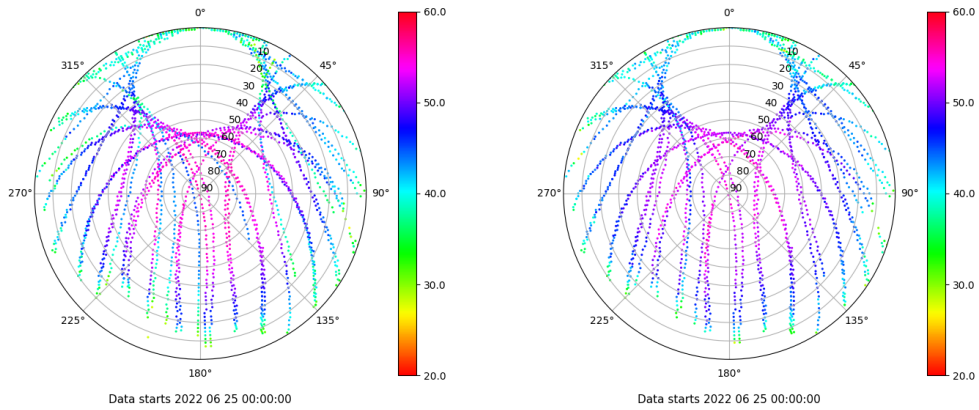
Skyplot for station YEBE. Signal to Noise S1C Data file YEBE00ESP_R_2022176.xtr Skyplot for station YEBE. Signal to Noise S2C Data file YEBE00ESP_R_2022176.xtr
