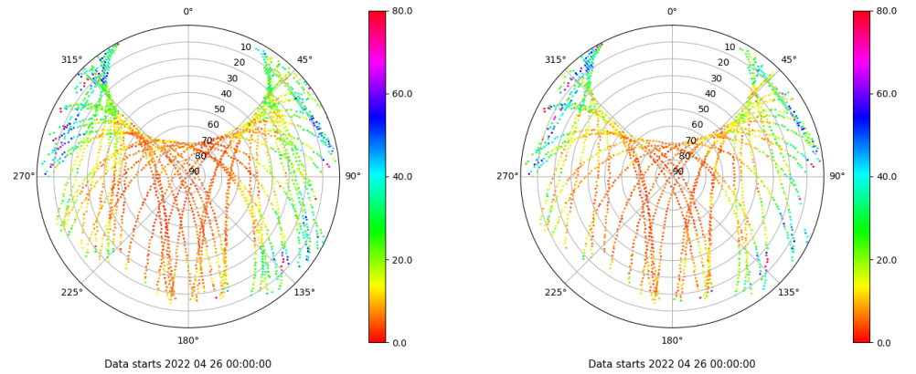
Skyplot for station YEBE. Parameter M1C Data file YEBE00ESP_R_2022116.xtr Skyplot for station YEBE. Parameter M2S Data file YEBE00ESP_R_2022116.xtr
