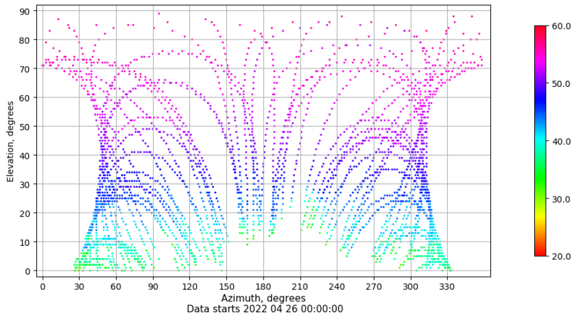
Azimuth-elevation plot for station YEBE. Signal to Noise S1C Data file YEBE00ESP_R_2022116.xtr
