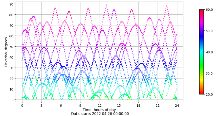
Time-elevation plot for station YEBE. Signal to Noise S1C Data file YEBE00ESP_R_2022116.xtr
