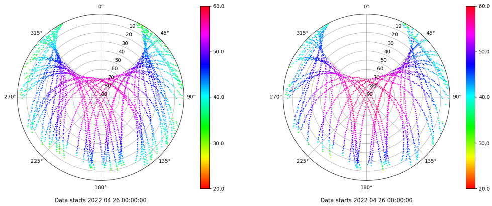
Skyplot for station YEBE. Signal to Noise S1C Data file YEBE00ESP_R_2022116.xtr Skyplot for station YEBE. Signal to Noise S2S Data file YEBE00ESP_R_2022116.xtr
