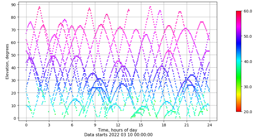
Time-elevation plot for station YEBE. Signal to Noise S1C Data file YEBE00ESP_R_2022069.xtr
