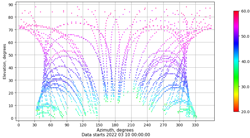
Azimuth-elevation plot for station YEBE. Signal to Noise S1C Data file YEBE00ESP_R_2022069.xtr
