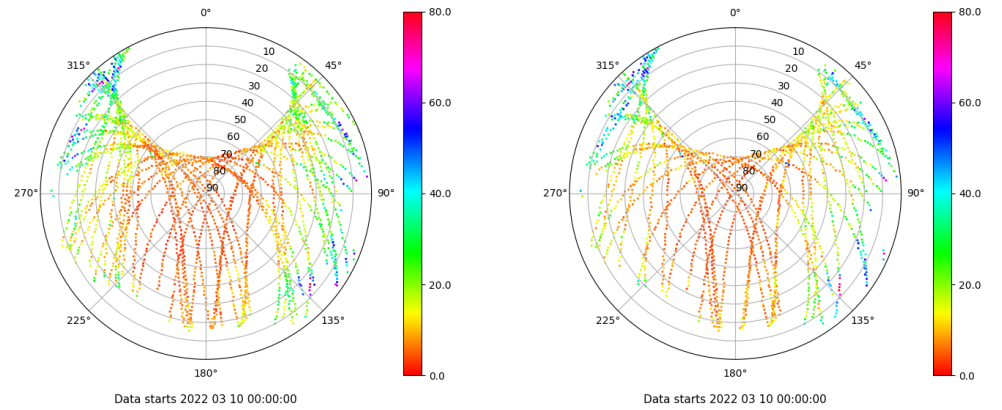
Skyplot for station YEBE. Parameter M1C Data file YEBE00ESP_R_2022069.xtr Skyplot for station YEBE. Parameter M2S Data file YEBE00ESP_R_2022069.xtr
