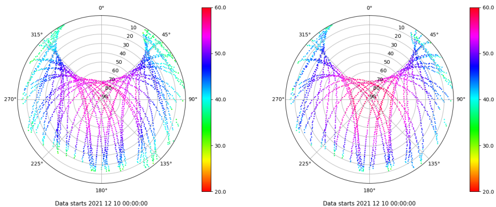
Skyplot for station YEBE. Signal to Noise S1C Data file YEBE00ESP_R_2021344.xtr Skyplot for station YEBE. Signal to Noise S2S Data file YEBE00ESP_R_2021344.xtr
