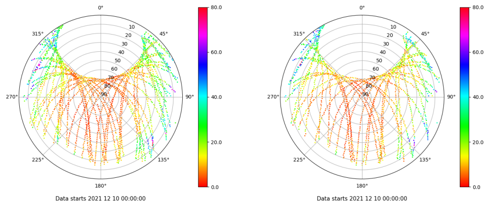
Skyplot for station YEBE. Parameter M1C Data file YEBE00ESP_R_2021344.xtr Skyplot for station YEBE. Parameter M2S Data file YEBE00ESP_R_2021344.xtr
