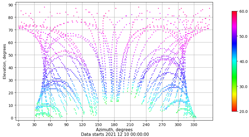
Azimuth-elevation plot for station YEBE. Signal to Noise S1C Data file YEBE00ESP_R_2021344.xtr
