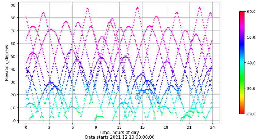
Time-elevation plot for station YEBE. Signal to Noise S1C Data file YEBE00ESP_R_2021344.xtr
