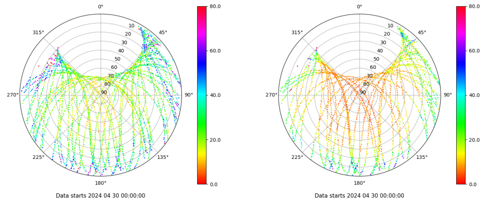
Skyplot for station YEB1. Parameter M1C Data file YEB100ESP_R_2024121.xtr Skyplot for station YEB1. Parameter M2S Data file YEB100ESP_R_2024121.xtr
