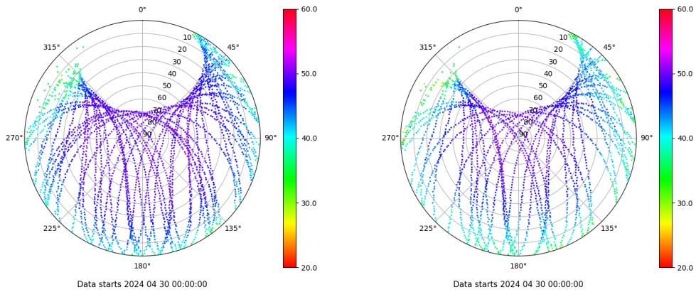
Skyplot for station YEB1. Signal to Noise S1C Data file YEB100ESP_R_2024121.xtr Skyplot for station YEB1. Signal to Noise S2S Data file YEB100ESP_R_2024121.xtr
