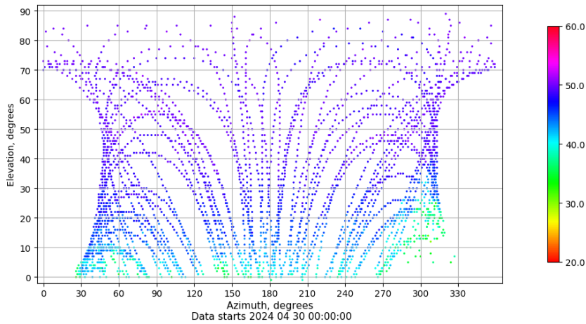
Azimuth-elevation plot for station YEB1. Signal to Noise S1C Data file YEB100ESP_R_2024121.xtr
