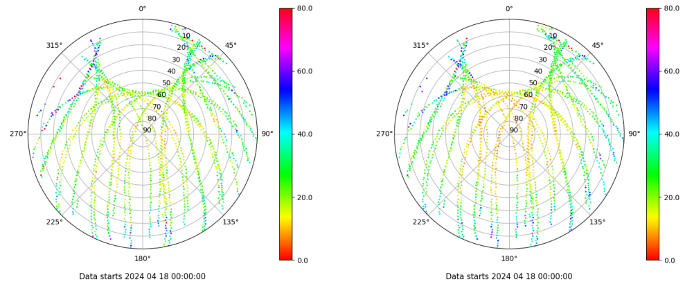
Skyplot for station YEB1. Parameter M1C Data file YEB100ESP_R_2024109.xtr Skyplot for station YEB1. Parameter M2P Data file YEB100ESP_R_2024109.xtr
