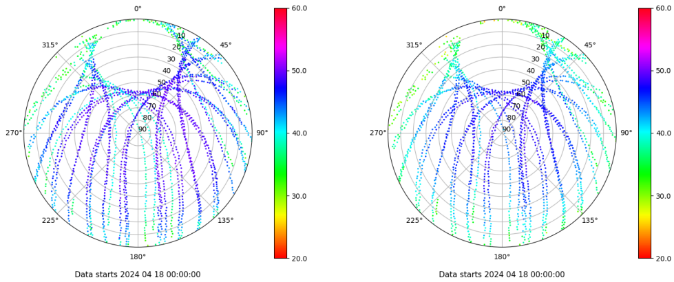
Skyplot for station YEB1. Signal to Noise S1C Data file YEB100ESP_R_2024109.xtr Skyplot for station YEB1. Signal to Noise S2P Data file YEB100ESP_R_2024109.xtr
