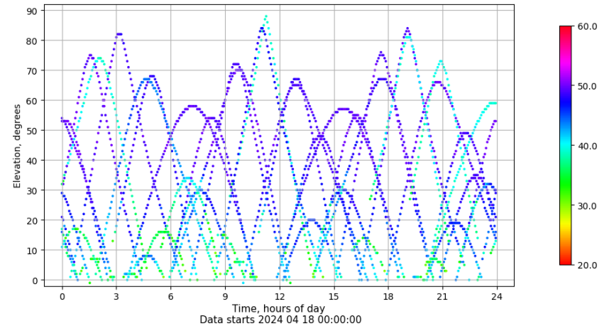
Time-elevation plot for station YEB1. Signal to Noise S1C Data file YEB100ESP_R_2024109.xtr
