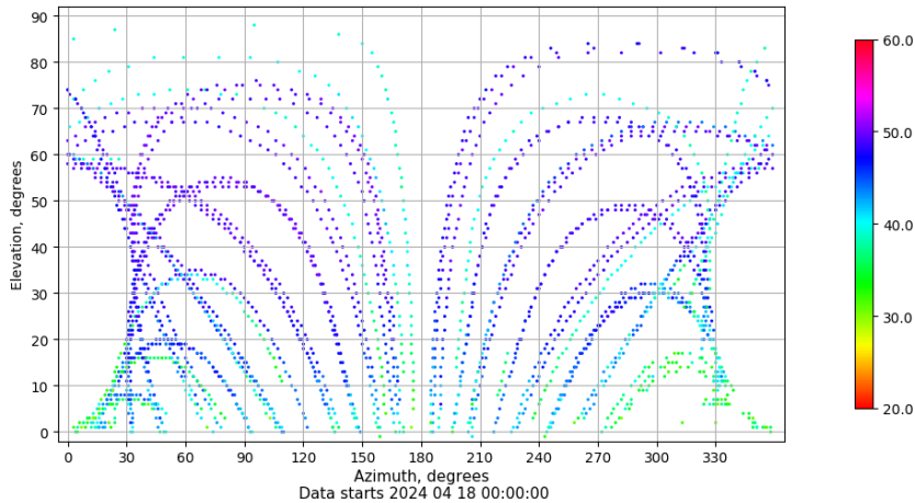
Azimuth-elevation plot for station YEB1. Signal to Noise S1C Data file YEB100ESP_R_2024109.xtr
