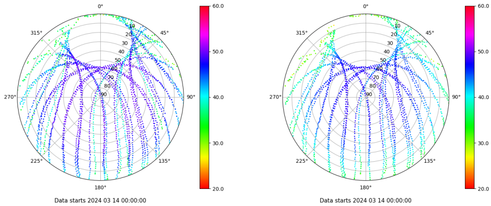
Skyplot for station YEB1. Signal to Noise S1C Data file YEB100ESP_R_2024074.xtr Skyplot for station YEB1. Signal to Noise S2P Data file YEB100ESP_R_2024074.xtr
