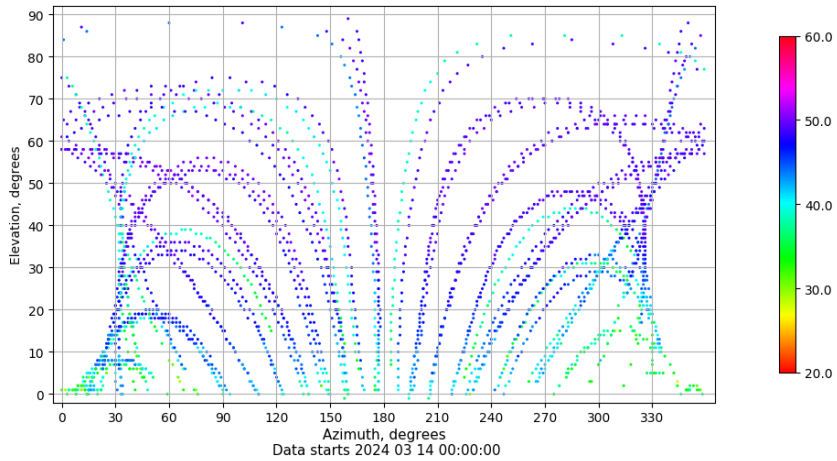
Azimuth-elevation plot for station YEB1. Signal to Noise S1C Data file YEB100ESP_R_2024074.xtr
