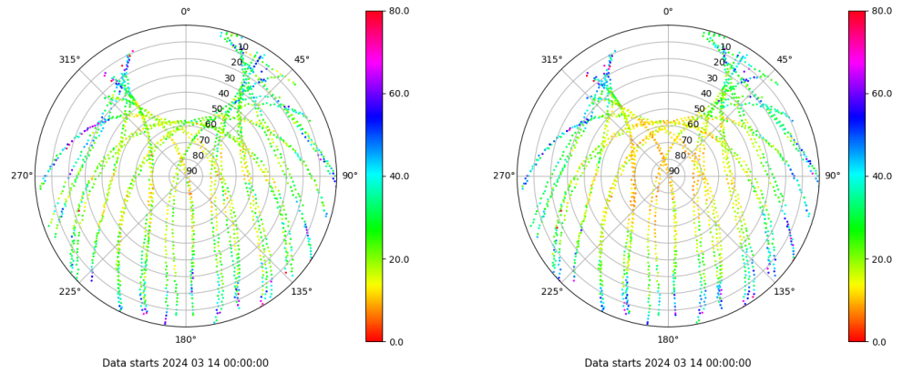
Skyplot for station YEB1. Parameter M1C Data file YEB100ESP_R_2024074.xtr Skyplot for station YEB1. Parameter M2P Data file YEB100ESP_R_2024074.xtr
