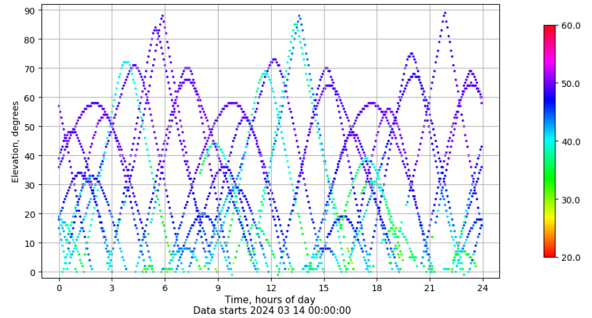
Time-elevation plot for station YEB1. Signal to Noise S1C Data file YEB100ESP_R_2024074.xtr
