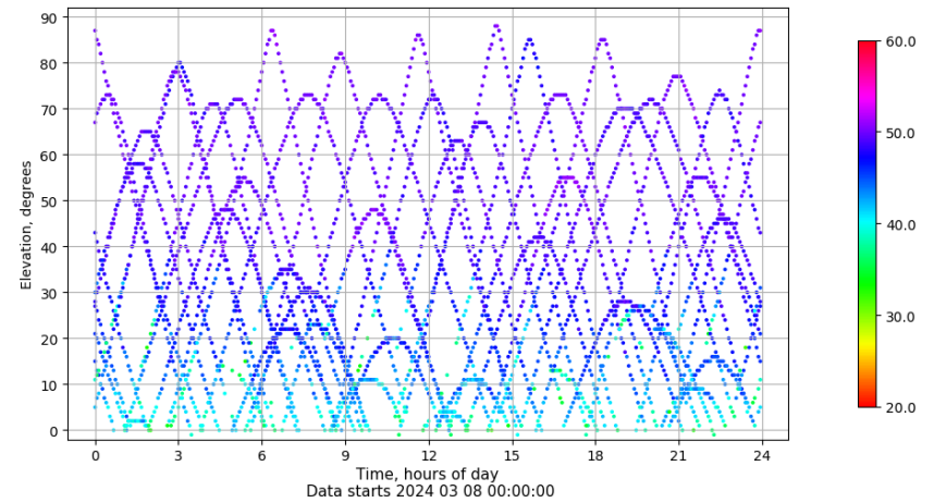
Time-elevation plot for station YEB1. Signal to Noise S1C Data file YEB100ESP_R_2024068.xtr
