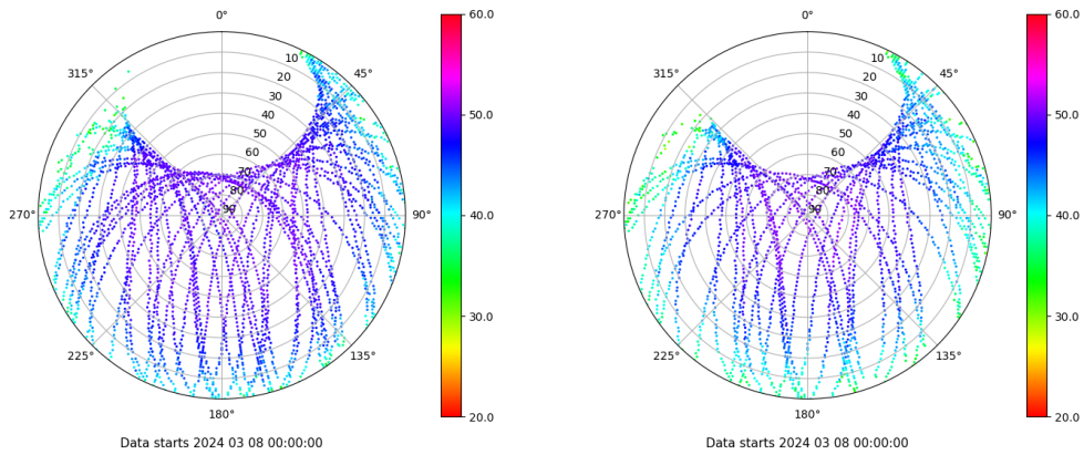
Skyplot for station YEB1. Signal to Noise S1C Data file YEB100ESP_R_2024068.xtr Skyplot for station YEB1. Signal to Noise S2S Data file YEB100ESP_R_2024068.xtr
