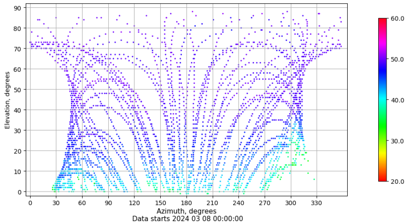
Azimuth-elevation plot for station YEB1. Signal to Noise S1C Data file YEB100ESP_R_2024068.xtr
