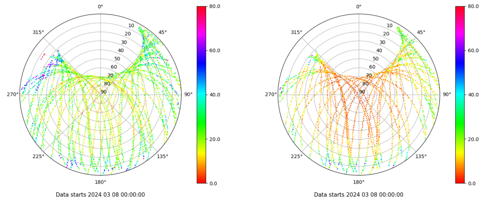
Skyplot for station YEB1. Parameter M1C Data file YEB100ESP_R_2024068.xtr Skyplot for station YEB1. Parameter M2S Data file YEB100ESP_R_2024068.xtr
