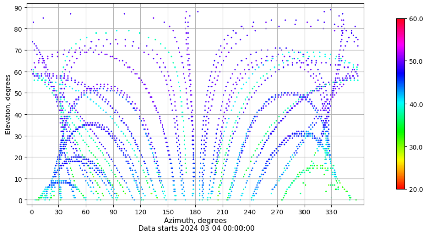
Azimuth-elevation plot for station YEB1. Signal to Noise S1C Data file YEB100ESP_R_2024064.xtr
