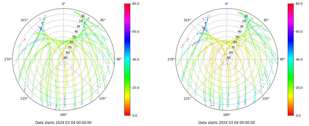
Skyplot for station YEB1. Parameter M1C Data file YEB100ESP_R_2024064.xtr Skyplot for station YEB1. Parameter M2P Data file YEB100ESP_R_2024064.xtr
