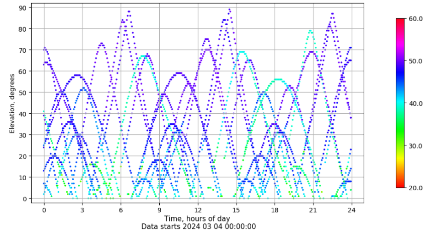
Time-elevation plot for station YEB1. Signal to Noise S1C Data file YEB100ESP_R_2024064.xtr
