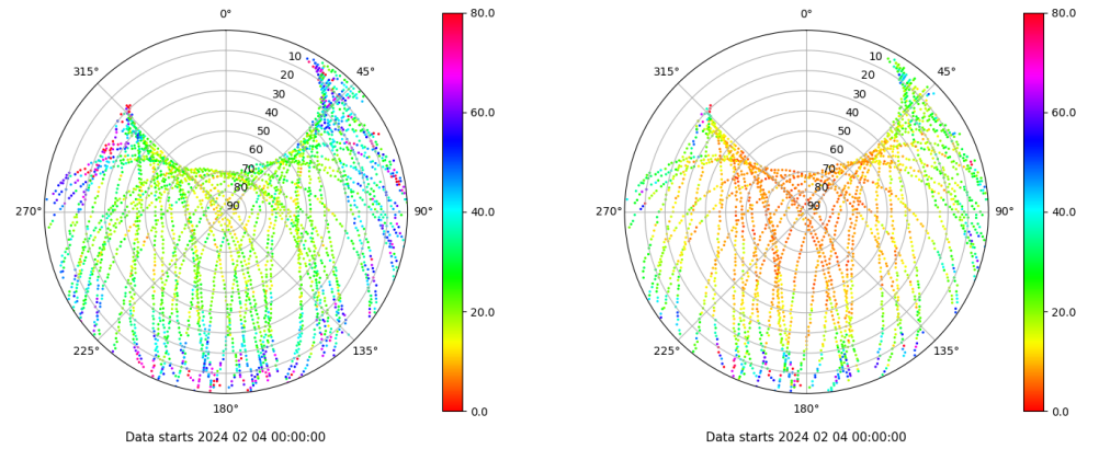
Skyplot for station YEB1. Parameter M1C Data file YEB100ESP_R_2024035.xtr Skyplot for station YEB1. Parameter M2S Data file YEB100ESP_R_2024035.xtr
