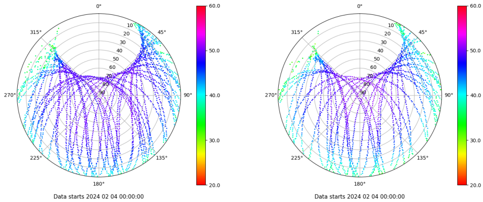
Skyplot for station YEB1. Signal to Noise S1C Data file YEB100ESP_R_2024035.xtr Skyplot for station YEB1. Signal to Noise S2S Data file YEB100ESP_R_2024035.xtr
