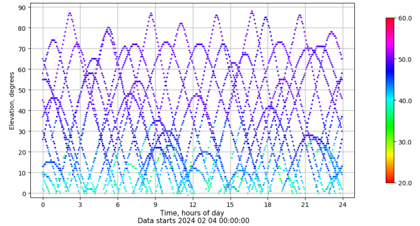
Time-elevation plot for station YEB1. Signal to Noise S1C Data file YEB100ESP_R_2024035.xtr
