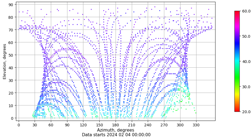
Azimuth-elevation plot for station YEB1. Signal to Noise S1C Data file YEB100ESP_R_2024035.xtr
