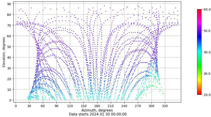
Azimuth-elevation plot for station YEB1. Signal to Noise S1C Data file YEB100ESP_R_2024030.xtr
