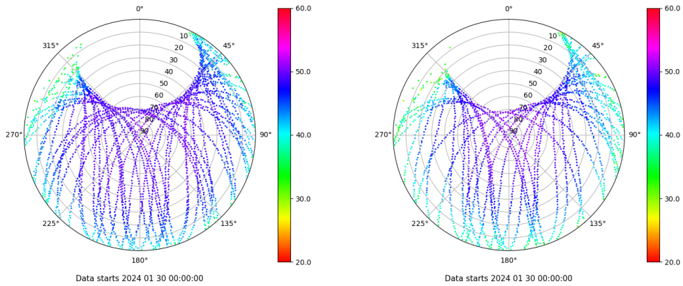
Skyplot for station YEB1. Signal to Noise S1C Data file YEB100ESP_R_2024030.xtr Skyplot for station YEB1. Signal to Noise S2S Data file YEB100ESP_R_2024030.xtr
