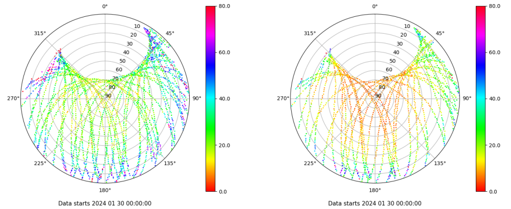
Skyplot for station YEB1. Parameter M1C Data file YEB100ESP_R_2024030.xtr Skyplot for station YEB1. Parameter M2S Data file YEB100ESP_R_2024030.xtr
