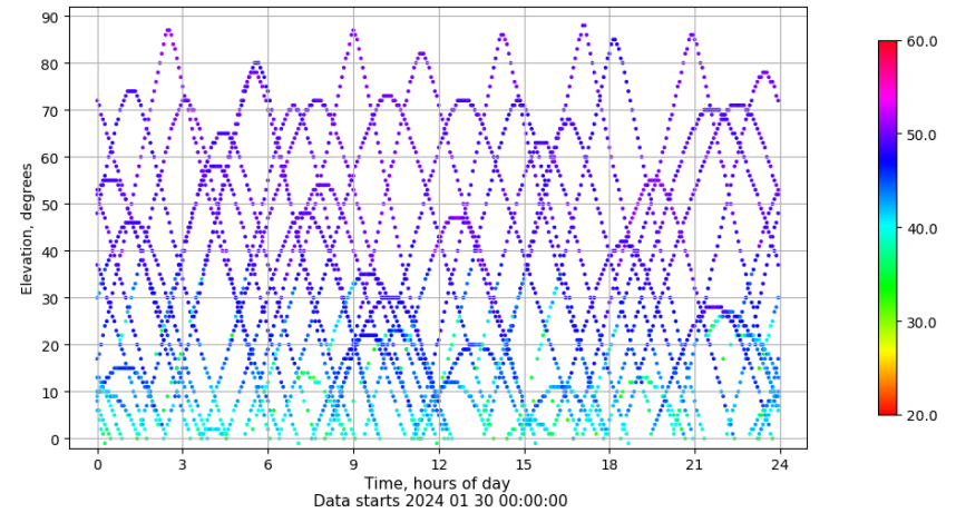
Time-elevation plot for station YEB1. Signal to Noise S1C Data file YEB100ESP_R_2024030.xtr
