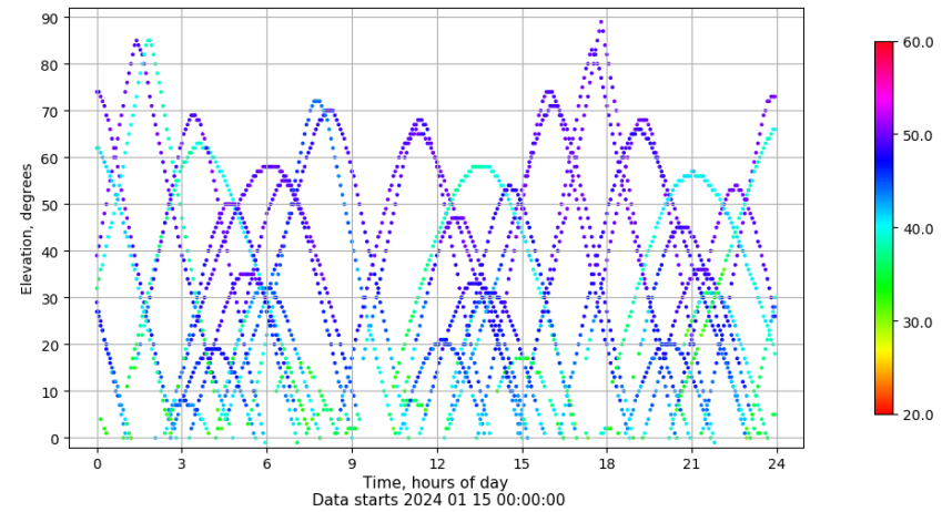
Time-elevation plot for station YEB1. Signal to Noise S1C Data file YEB100ESP_R_2024015.xtr
