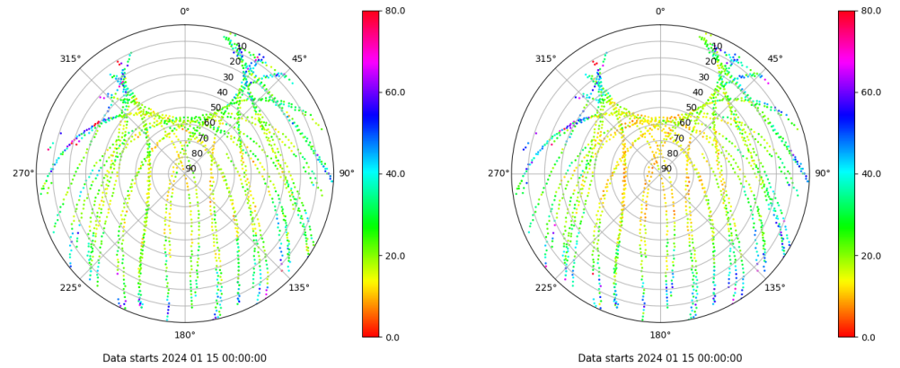
Skyplot for station YEB1. Parameter M1C Data file YEB100ESP_R_2024015.xtr Skyplot for station YEB1. Parameter M2P Data file YEB100ESP_R_2024015.xtr
