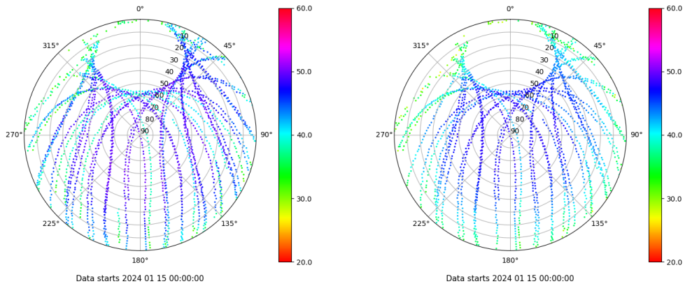
Skyplot for station YEB1. Signal to Noise S1C Data file YEB100ESP_R_2024015.xtr Skyplot for station YEB1. Signal to Noise S2P Data file YEB100ESP_R_2024015.xtr
