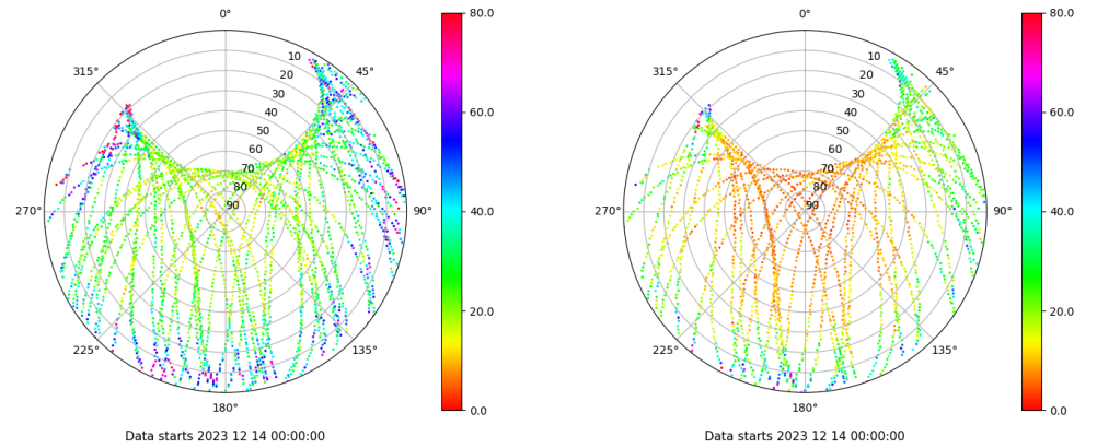
Skyplot for station YEB1. Parameter M1C Data file YEB100ESP_R_2023348.xtr Skyplot for station YEB1. Parameter M2S Data file YEB100ESP_R_2023348.xtr
