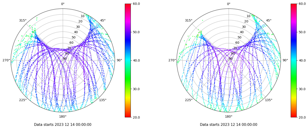
Skyplot for station YEB1. Signal to Noise S1C Data file YEB100ESP_R_2023348.xtr Skyplot for station YEB1. Signal to Noise S2S Data file YEB100ESP_R_2023348.xtr
