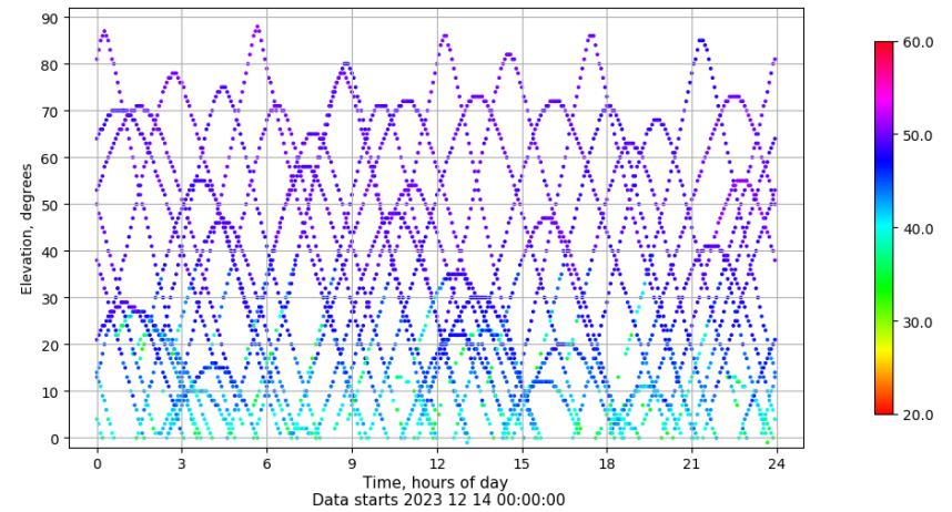
Time-elevation plot for station YEB1. Signal to Noise S1C Data file YEB100ESP_R_2023348.xtr
