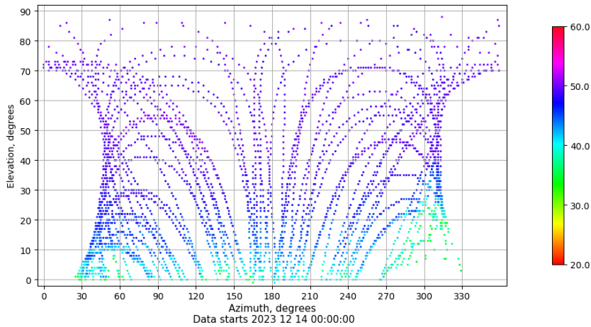
Azimuth-elevation plot for station YEB1. Signal to Noise S1C Data file YEB100ESP_R_2023348.xtr
