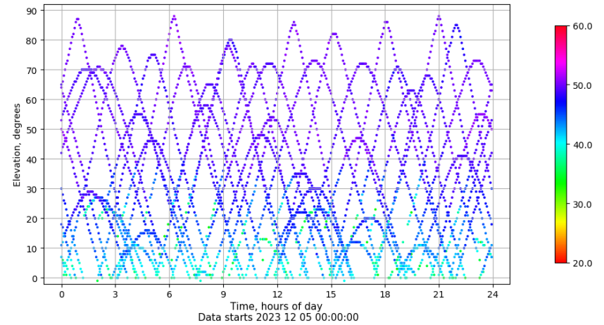
Time-elevation plot for station YEB1. Signal to Noise S1C Data file YEB100ESP_R_2023339.xtr
