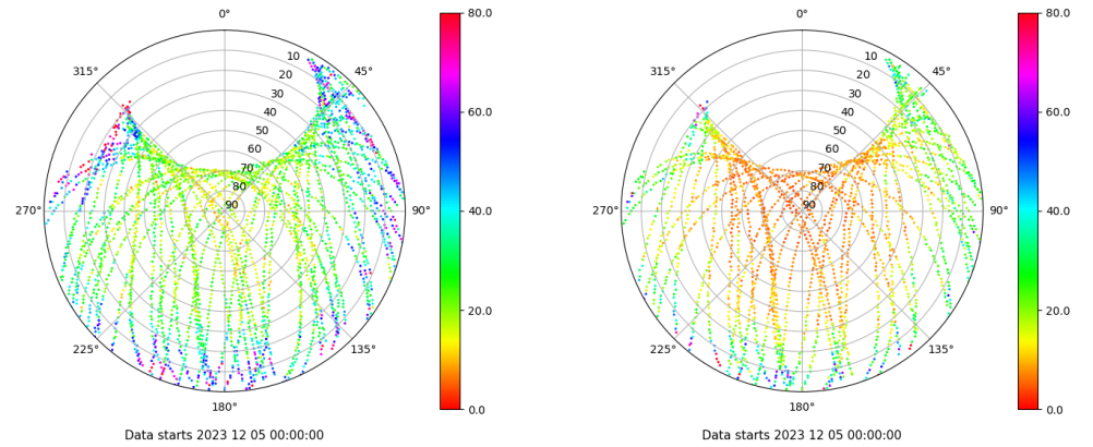
Skyplot for station YEB1. Parameter M1C Data file YEB100ESP_R_2023339.xtr Skyplot for station YEB1. Parameter M2S Data file YEB100ESP_R_2023339.xtr
