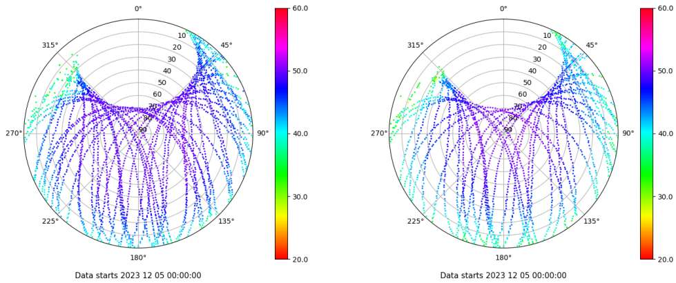
Skyplot for station YEB1. Signal to Noise S1C Data file YEB100ESP_R_2023339.xtr Skyplot for station YEB1. Signal to Noise S2S Data file YEB100ESP_R_2023339.xtr
