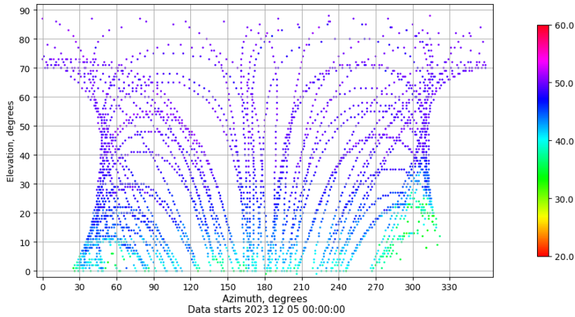
Azimuth-elevation plot for station YEB1. Signal to Noise S1C Data file YEB100ESP_R_2023339.xtr
