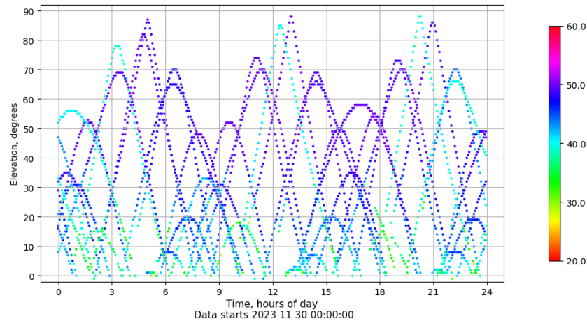
Time-elevation plot for station YEB1. Signal to Noise S1C Data file YEB100ESP_R_2023334.xtr
