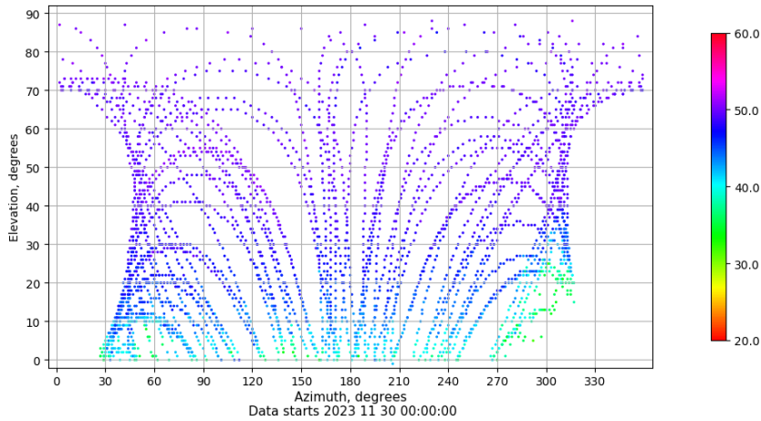
Azimuth-elevation plot for station YEB1. Signal to Noise S1C Data file YEB100ESP_R_2023334.xtr
