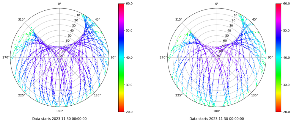
Skyplot for station YEB1. Signal to Noise S1C Data file YEB100ESP_R_2023334.xtr Skyplot for station YEB1. Signal to Noise S2S Data file YEB100ESP_R_2023334.xtr
