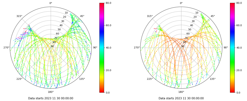
Skyplot for station YEB1. Parameter M1C Data file YEB100ESP_R_2023334.xtr Skyplot for station YEB1. Parameter M2S Data file YEB100ESP_R_2023334.xtr
