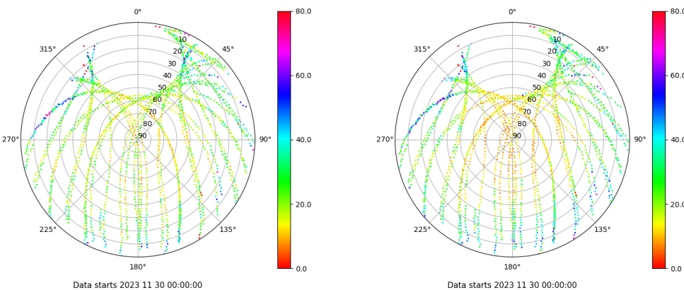
Skyplot for station YEB1. Parameter M1C Data file YEB100ESP_R_2023334.xtr Skyplot for station YEB1. Parameter M2P Data file YEB100ESP_R_2023334.xtr
