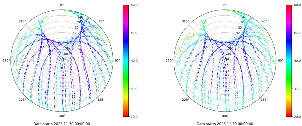
Skyplot for station YEB1. Signal to Noise S1C Data file YEB100ESP_R_2023334.xtr Skyplot for station YEB1. Signal to Noise S2P Data file YEB100ESP_R_2023334.xtr
