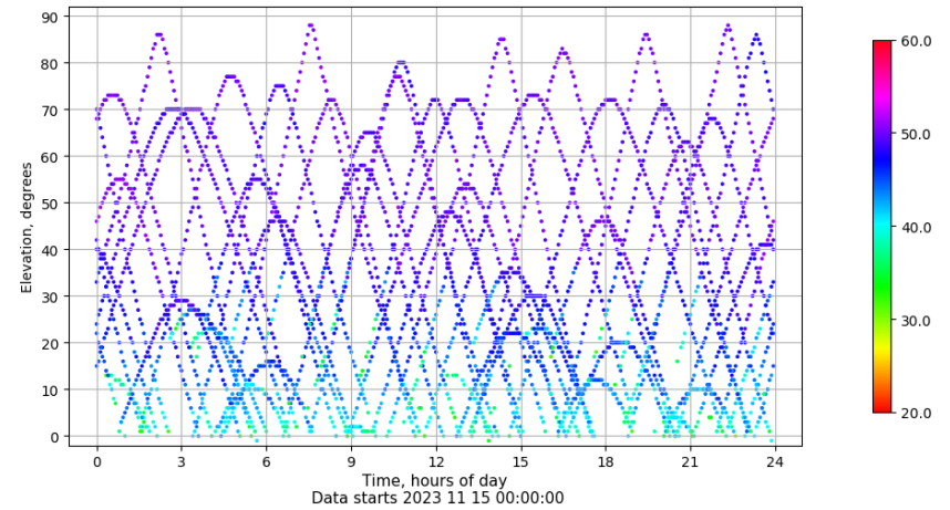
Time-elevation plot for station YEB1. Signal to Noise S1C Data file YEB100ESP_R_2023319.xtr
