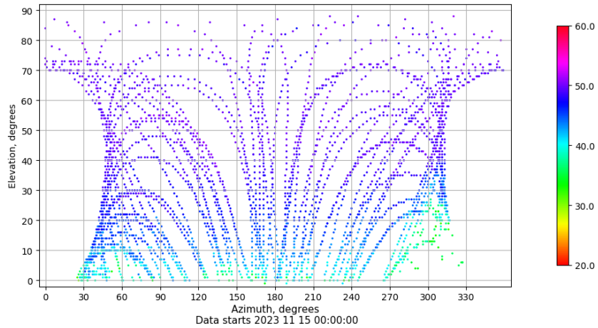
Azimuth-elevation plot for station YEB1. Signal to Noise S1C Data file YEB100ESP_R_2023319.xtr
