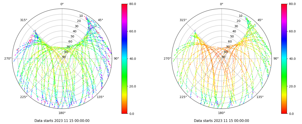
Skyplot for station YEB1. Parameter M1C Data file YEB100ESP_R_2023319.xtr Skyplot for station YEB1. Parameter M2S Data file YEB100ESP_R_2023319.xtr
