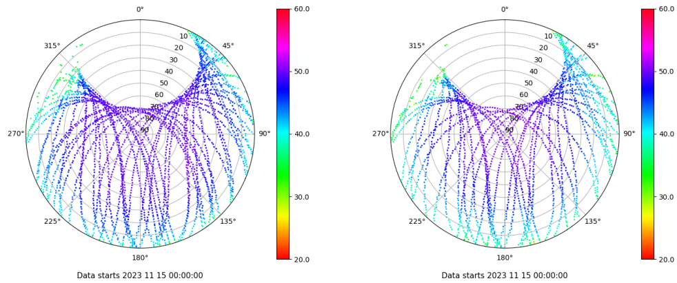
Skyplot for station YEB1. Signal to Noise S1C Data file YEB100ESP_R_2023319.xtr Skyplot for station YEB1. Signal to Noise S2S Data file YEB100ESP_R_2023319.xtr
