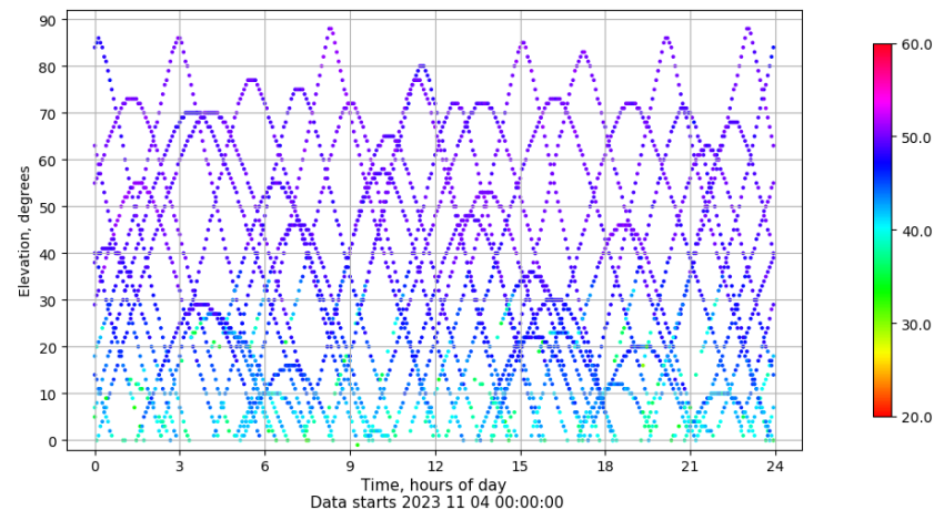
Time-elevation plot for station YEB1. Signal to Noise S1C Data file YEB100ESP_R_2023308.xtr
