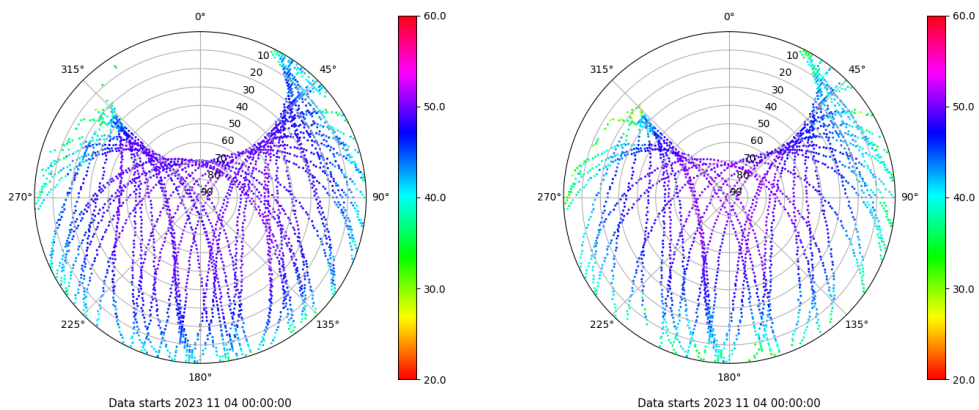
Skyplot for station YEB1. Signal to Noise S1C Data file YEB100ESP_R_2023308.xtr Skyplot for station YEB1. Signal to Noise S2S Data file YEB100ESP_R_2023308.xtr
