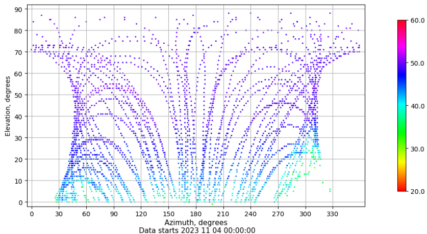
Azimuth-elevation plot for station YEB1. Signal to Noise S1C Data file YEB100ESP_R_2023308.xtr
