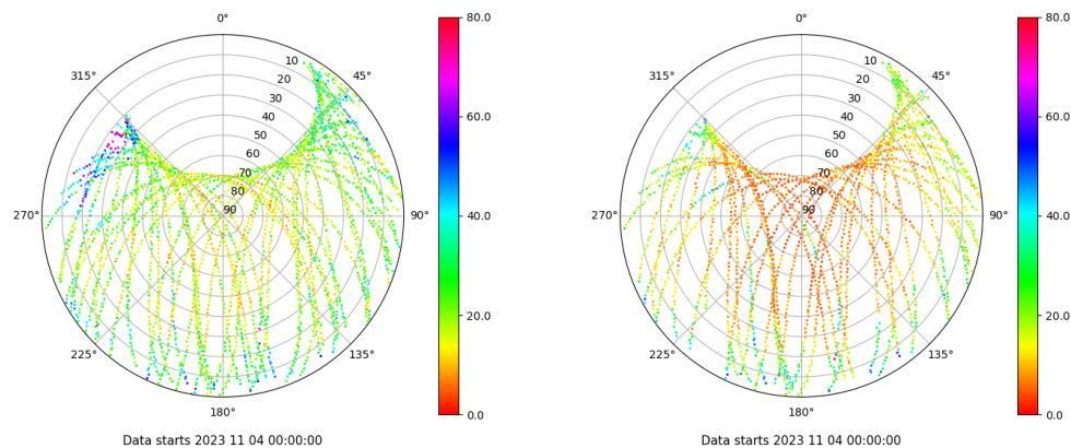
Skyplot for station YEB1. Parameter M1C Data file YEB100ESP_R_2023308.xtr Skyplot for station YEB1. Parameter M2S Data file YEB100ESP_R_2023308.xtr
