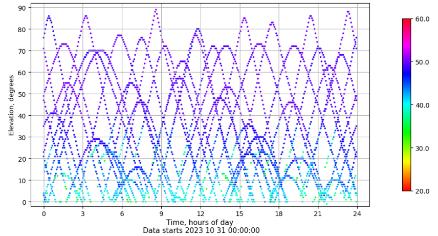
Time-elevation plot for station YEB1. Signal to Noise S1C Data file YEB100ESP_R_2023304.xtr
