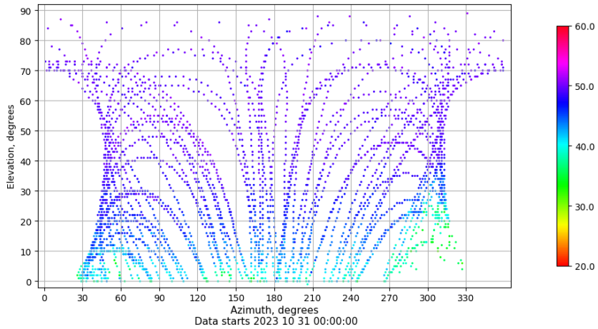
Azimuth-elevation plot for station YEB1. Signal to Noise S1C Data file YEB100ESP_R_2023304.xtr
