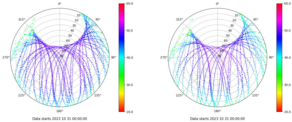
Skyplot for station YEB1. Signal to Noise S1C Data file YEB100ESP_R_2023304.xtr Skyplot for station YEB1. Signal to Noise S2S Data file YEB100ESP_R_2023304.xtr
