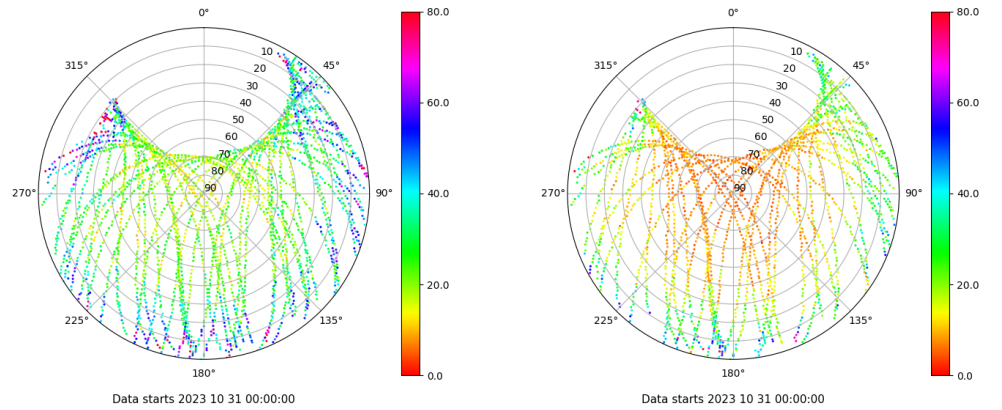
Skyplot for station YEB1. Parameter M1C Data file YEB100ESP_R_2023304.xtr Skyplot for station YEB1. Parameter M2S Data file YEB100ESP_R_2023304.xtr
