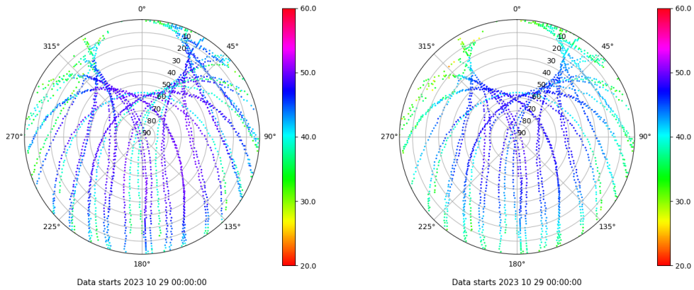
Skyplot for station YEB1. Signal to Noise S1C Data file YEB100ESP_R_2023302.xtr Skyplot for station YEB1. Signal to Noise S2P Data file YEB100ESP_R_2023302.xtr
