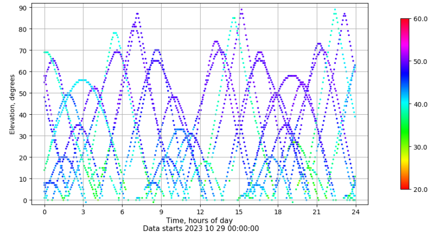
Time-elevation plot for station YEB1. Signal to Noise S1C Data file YEB100ESP_R_2023302.xtr
