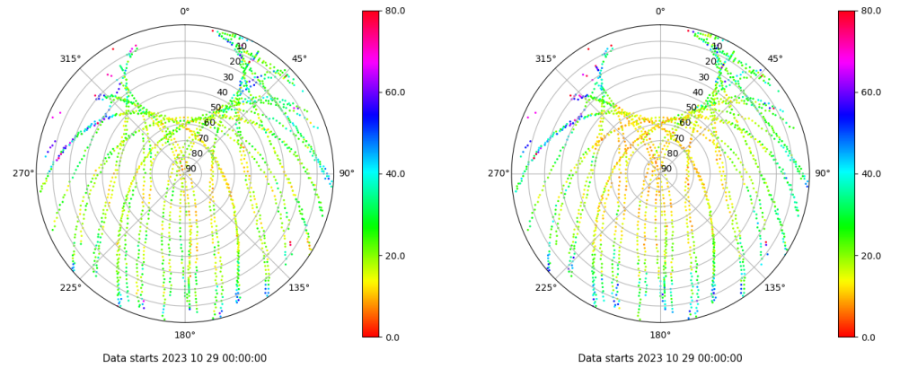
Skyplot for station YEB1. Parameter M1C Data file YEB100ESP_R_2023302.xtr Skyplot for station YEB1. Parameter M2P Data file YEB100ESP_R_2023302.xtr
