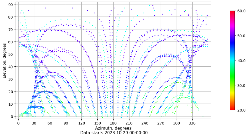
Azimuth-elevation plot for station YEB1. Signal to Noise S1C Data file YEB100ESP_R_2023302.xtr
