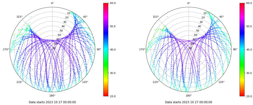
Skyplot for station YEB1. Signal to Noise S1C Data file YEB100ESP_R_2023300.xtr Skyplot for station YEB1. Signal to Noise S2S Data file YEB100ESP_R_2023300.xtr
