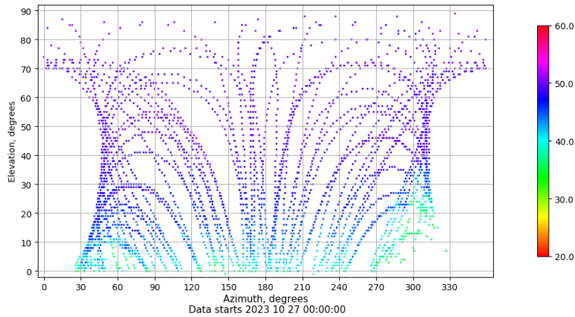
Azimuth-elevation plot for station YEB1. Signal to Noise S1C Data file YEB100ESP_R_2023300.xtr
