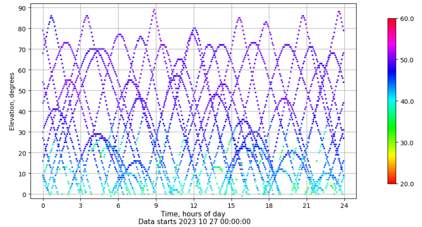
Time-elevation plot for station YEB1. Signal to Noise S1C Data file YEB100ESP_R_2023300.xtr
