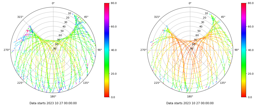
Skyplot for station YEB1. Parameter M1C Data file YEB100ESP_R_2023300.xtr Skyplot for station YEB1. Parameter M2S Data file YEB100ESP_R_2023300.xtr
