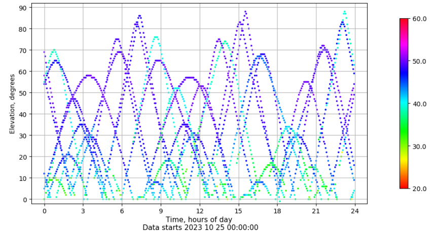
Time-elevation plot for station YEB1. Signal to Noise S1C Data file YEB100ESP_R_2023298.xtr
