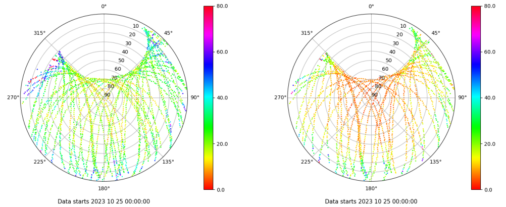
Skyplot for station YEB1. Parameter M1C Data file YEB100ESP_R_2023298.xtr Skyplot for station YEB1. Parameter M2S Data file YEB100ESP_R_2023298.xtr
