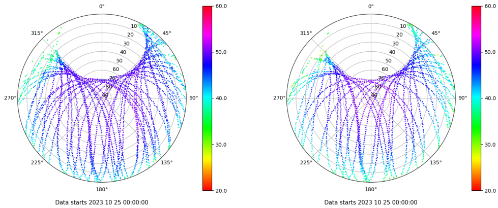
Skyplot for station YEB1. Signal to Noise S1C Data file YEB100ESP_R_2023298.xtr Skyplot for station YEB1. Signal to Noise S2S Data file YEB100ESP_R_2023298.xtr
