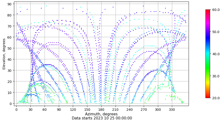
Azimuth-elevation plot for station YEB1. Signal to Noise S1C Data file YEB100ESP_R_2023298.xtr
