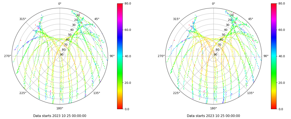
Skyplot for station YEB1. Parameter M1C Data file YEB100ESP_R_2023298.xtr Skyplot for station YEB1. Parameter M2P Data file YEB100ESP_R_2023298.xtr
