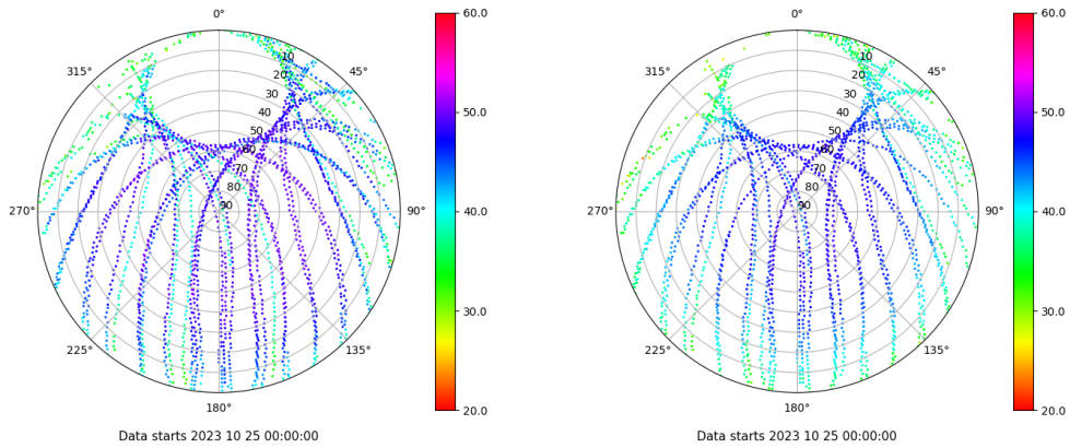
Skyplot for station YEB1. Signal to Noise S1C Data file YEB100ESP_R_2023298.xtr Skyplot for station YEB1. Signal to Noise S2P Data file YEB100ESP_R_2023298.xtr
